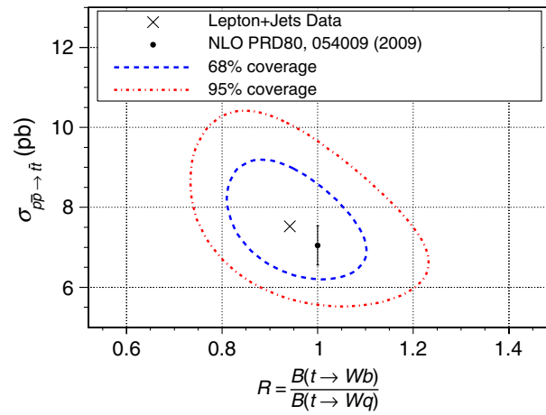
FIG. 2 (color online). The fit results for the simultaneous measurement of R and \sigma_{t\bar{t}} . The X-cross corresponds to the maximum of the likelihood; the point with error bar to the NLO cross section calculation. The two-dimensional confidence regions are shown as well.
