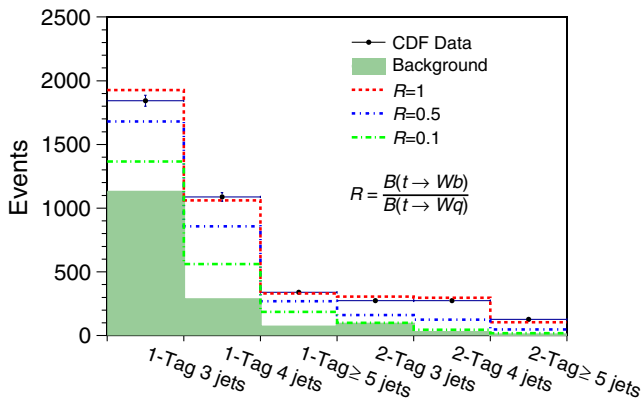
FIG. 1 (color online). Observed events for the analysis final states after summing over lepton categories, compared to expected events for different values of R . For the t\bar{t} normalization the theoretical value \sigma_{t\bar{t}} = 7.04 \pm 0.49 pb is used.
