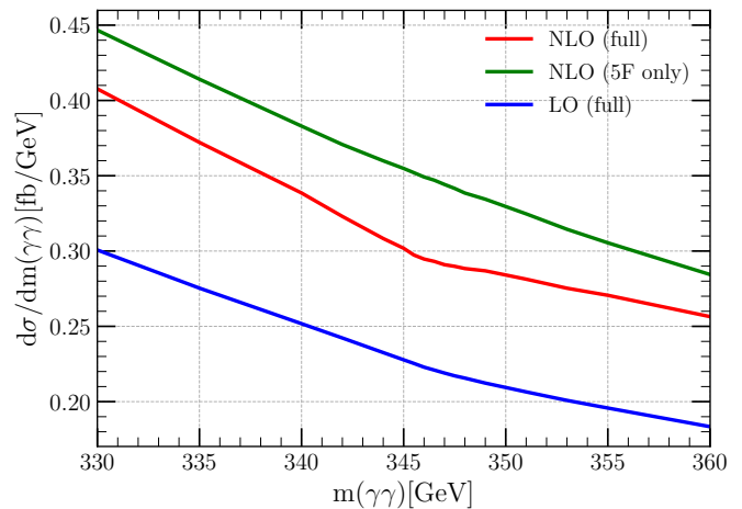
FIG. 3. The differential cross section before and after including the top-quark contribution is shown for the top pair threshold region.
