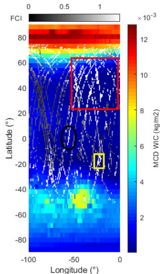
Figure 9. Comparison between the FCI results (grey scale) with the MCD Water Ice Column (colour scale) for all latitudes and longitude from 100°W to 0°. Grey scale: LNO observations in MY35, from L_S 30° to 150°. Saturated FCI values are in white ( >3.5\sigma , see Section 4.1). Colour scale: MCD Water ice column simulation for L_S 150° and 15 LTST.
