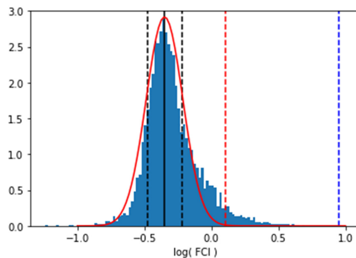
Figure 5. FCI values distribution in logarithmic X-scale for MY34-35. Solid black line: mean value of the distribution ( \mu = -0.35 ). Dashed black line: standard deviation of the distribution ( \sigma = 0.13 ). Dashed red line: mean value of FCI at the polar cap edge ( \mu + 3.5\sigma ). Dashed blue line: mean value of FCI on the polar cap deposits ( \mu + 10\sigma ).
