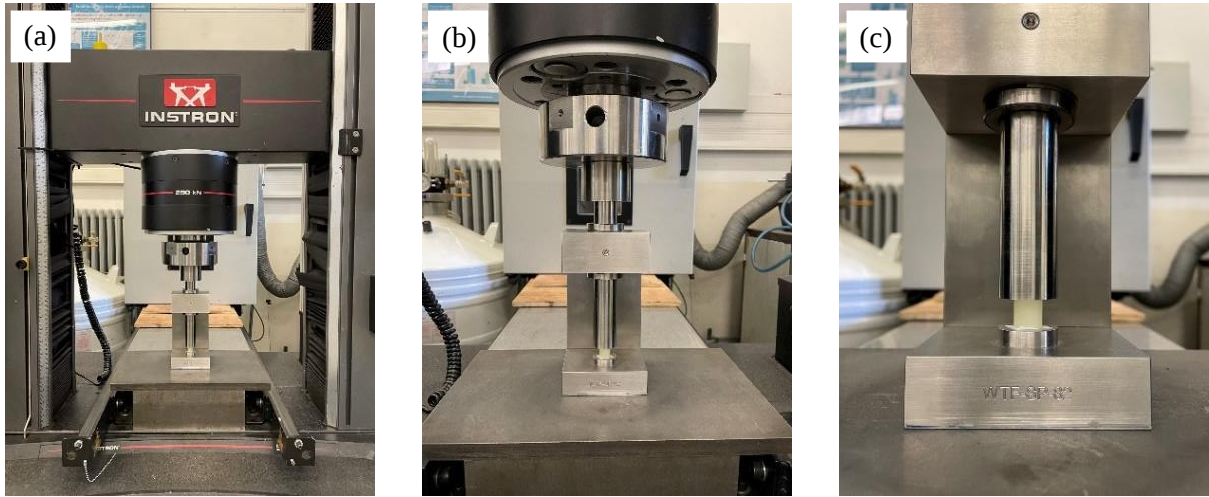
Figure 1. Testing apparatus and specimen: (a) Instron 5985 testing machine; (b) subpress from Wyoming Test Fixtures (WTF-SP); (c) specimen and PTFE films.
