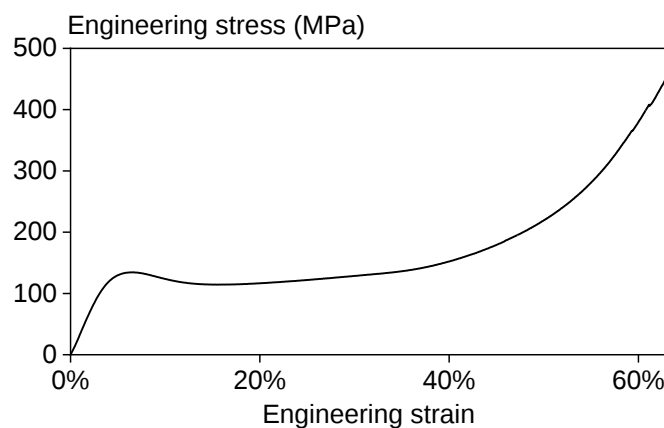
(a) Engineering stress-strain curve
