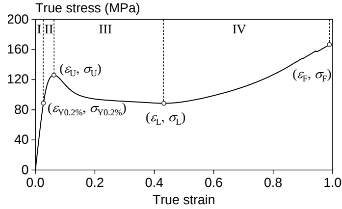
(b) True stress-strain curve
