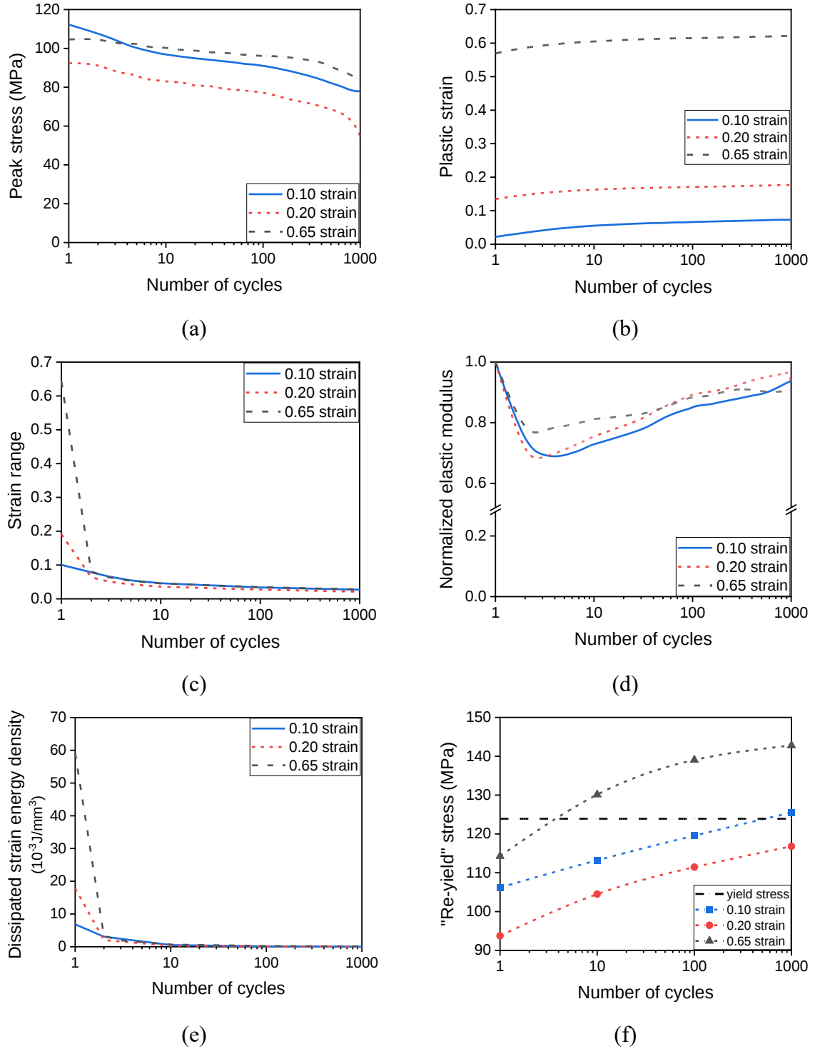
Figure 4. The evolution of (a) peak stress, (b) plastic strain, (c) strain range, (d) normalised elastic modulus, (e) dissipated strain energy density per cycle, and (f) 're-yield' stress as a function of the number of loading cycles compared to the nominal value of the yield strength prior to cyclic loading.
