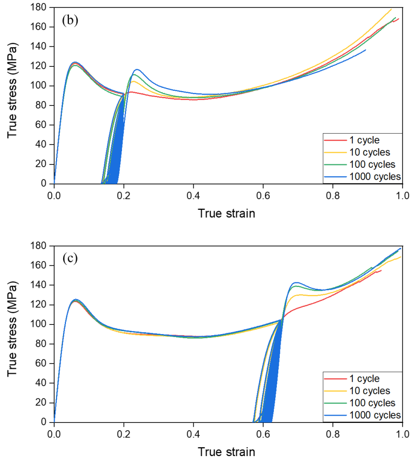
Figure 5. True stress-strain curves for (a) 0.10, (b) 0.20, and (c) 0.65 applied peak strain.
