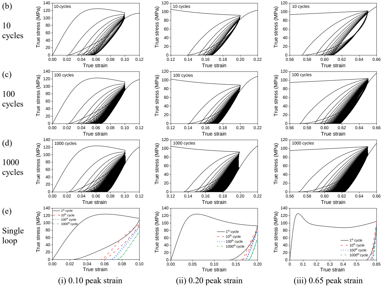
Figure 3. Hysteresis loop of (i) 0.10, (ii) 0.20 and (iii) 0.65 peak strains for (a) 1 cycle, (b) 10 cycles, (c) 100 cycles and (d) 1000 cycles; (e) single loop.
