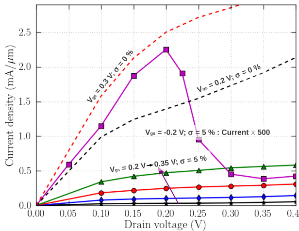
Figure 5. I - V_{ds} characteristics of simulated graphene nFETs with different V_{gs} : unstrained graphene channel ( \sigma = 0\% ) and strained graphene heterostructure ( \sigma = 5\% ). Note that the current at V_{gs} = -0.2 V is multiplied by 500.
