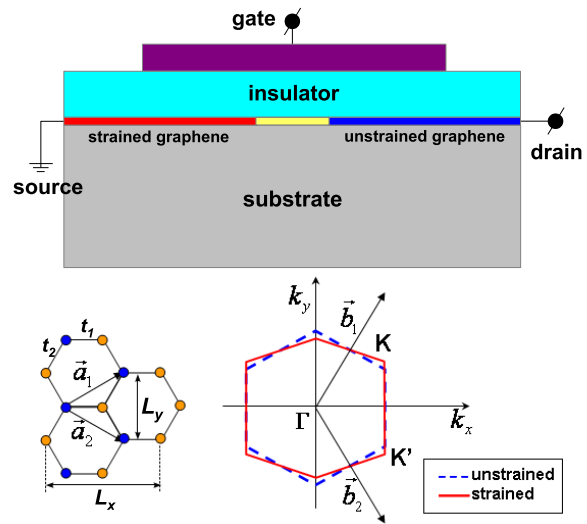
Figure 1. Schematic of the graphene FETs simulated in this work (top) and a graphene lattice together with its first Brillouin zone (bottom). The channel of the simulated device is based on strained graphene heterostructures. The yellow zone in the top figure indicates the transition region between strained and unstrained sections. At the bottom, the left panel shows the honeycomb structure with the lattice vectors \vec{a}_1 and \vec{a}_2 . L_{x,y} are the lengths of the unit cell (four atoms per cell) along the Ox and Oy directions, respectively. The right panel shows the Brillouin zones, showing the change in Dirac points ( K and K' ) with uniaxial strains applied along the Ox -axis (transport direction).
