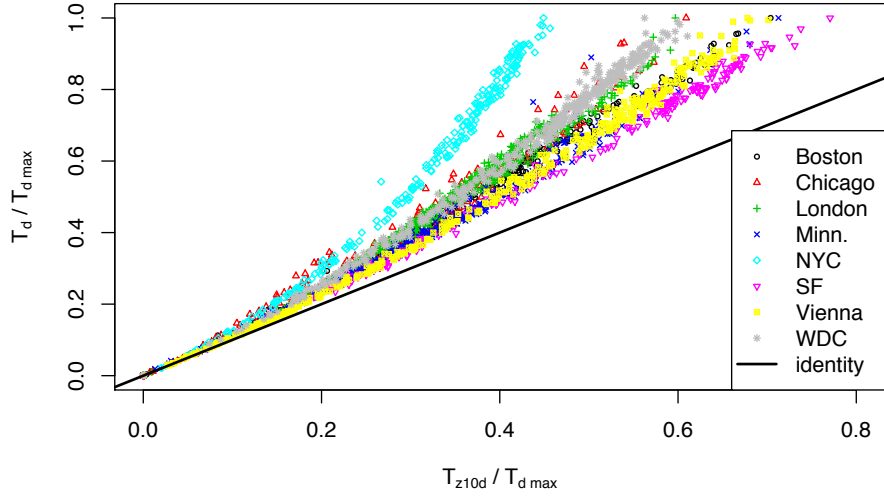
Figure 3.3: Normalized T_d plotted against T_{z10d} for the eight case studies showing the amounts of interaction collisions.
