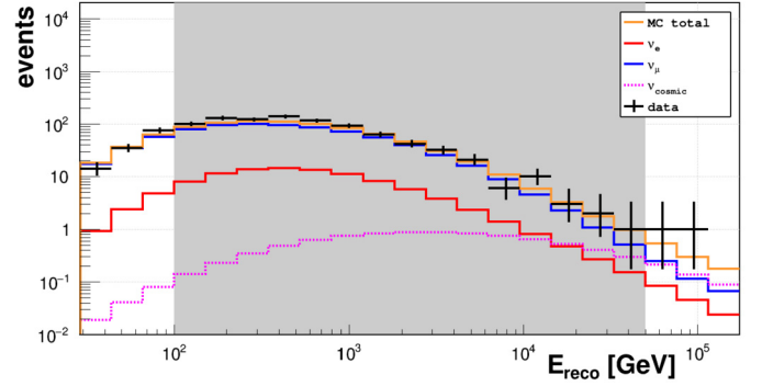
Fig. 2. Distribution of E_{\text{reco}} with the binning used for the construction of the response matrix for the \nu_\mu sample (blue histogram). The red histogram, with the same binning, refers to the \nu_e sample. The magenta histogram is the expected contribution from a cosmic neutrino flux, as estimated in [28], while the orange histogram includes the sum of all MC contributions. The black crosses correspond to real data. Events in the shaded region are used for unfolding.
