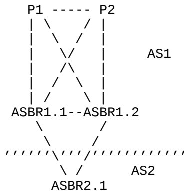
Figure 5. IBGP Full-Mesh
