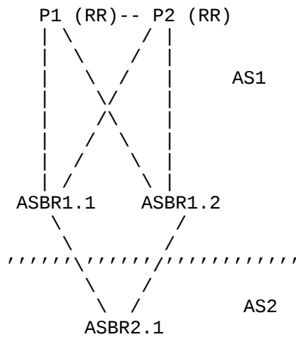
Figure 6. Route Reflector
