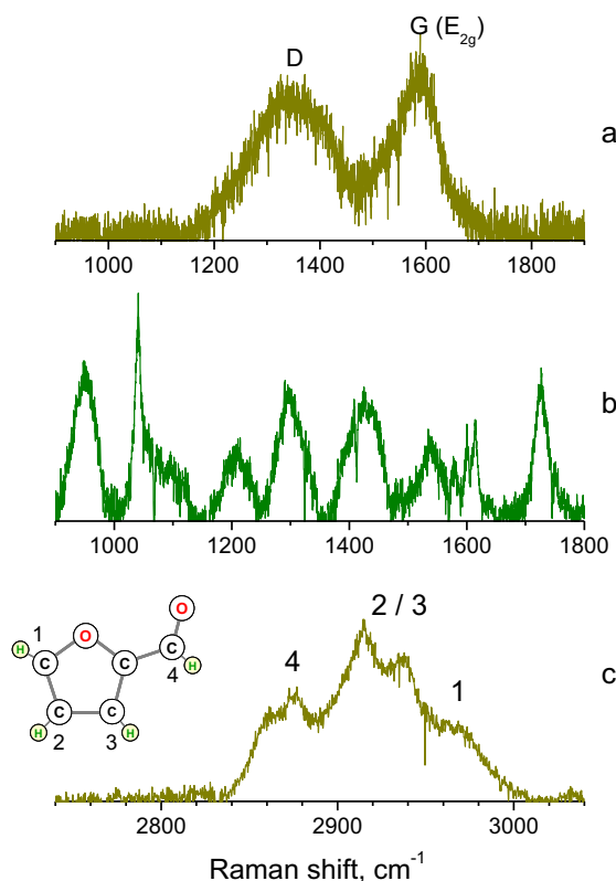
Fig. 6. Raman spectra of the black (a) and white (b,c) solid products collected after the photocatalytic process followed by the photocatalyst heating at 400 °C.
