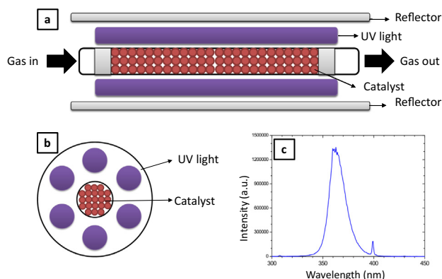
Fig. 1. (a) Cut section and (b) cross section of the photocatalytic reactor and (c) Emission spectrum of the UV light.
