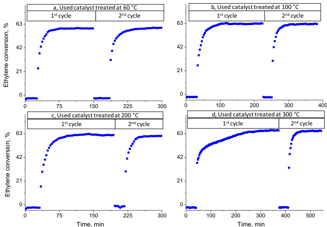
Fig. 3. Ethylene conversion of used Fe(III)-TiO 2 photocatalyst subsequently heat treated in a dry air flow: (a) at 60 °C during 3 h under UVA illumination, (b) at 100 °C during 3 h, (c) at 200 °C during 3 h and d) at 300 °C during 1 h. (Each photocatalyst has been studied in two repeated cycles).
