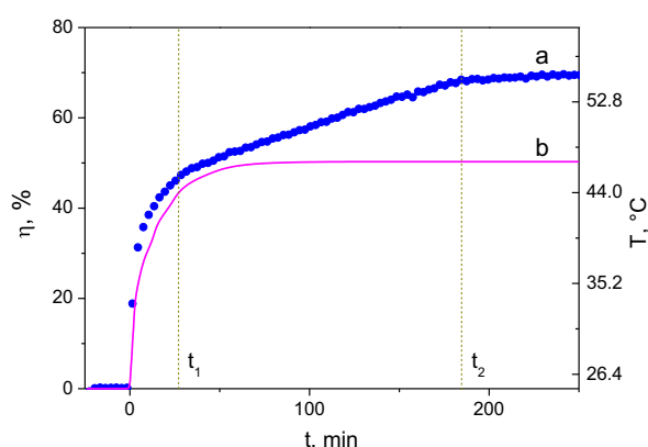
Fig. 2. Ethylene conversion \eta (a) and temperature (b) of a fixed-bed continuous-flow photocatalytic reactor.
