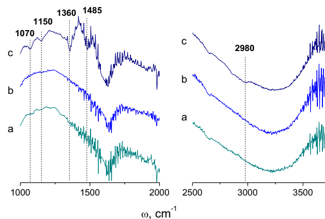
Fig. 4. FTIR spectra of Fe(III)-TiO 2 photocatalyst (a) freshly prepared, (b) freshly prepared after being exposed to gaseous ethylene flow in dark for 3 h and (c) after UVA illumination in presence of pollutant for 3 h.
