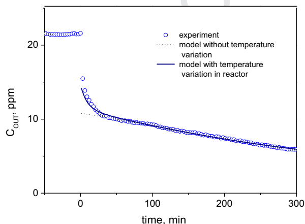
Fig. 7. Ethylene concentration at the photocatalytic reactor exit versus time (experiment and modelling).
