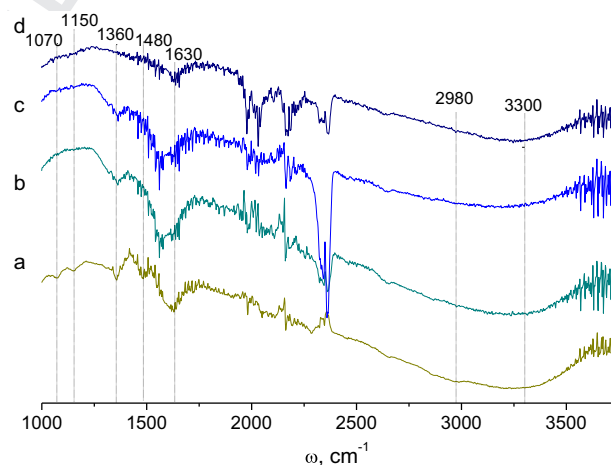
Fig. 5. FTIR spectra of Fe(III)-TiO 2 photocatalyst: freshly prepared (a) and used after secondary thermal treatment for 1 h at 100 °C (b), 200 °C (c) and 300 °C (d).
