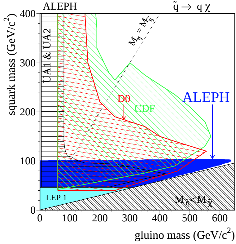
Figure 6: Excluded regions at 95% C.L. from the search for generic \tilde{q}\tilde{q} pairs, assuming five mass-degenerate \tilde{q} flavours. The results are shown in the gluino-squark mass plane for \tan\beta = 4 and \mu = -400 \text{ GeV} , together with results from experiments at p\bar{p} colliders.
