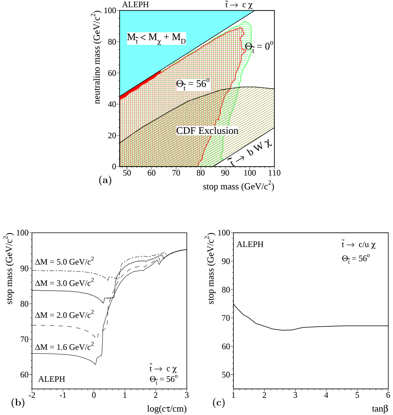
Figure 2: (a) Excluded regions at 95% C.L. in the M_\chi vs M_{\tilde{t}} plane from \tilde{t} \rightarrow c/u \chi searches; the excluded regions are given for \theta_{\tilde{t}} = 0^\circ , corresponding to maximum \tilde{t}\tilde{t}Z coupling, and for \theta_{\tilde{t}} = 56^\circ , corresponding to vanishing \tilde{t}\tilde{t}Z coupling. The dark region in the small \Delta M corridor is excluded by the “long-lived hadrons” analysis. The CDF experiment result is also indicated. (b) Stop mass lower limit at 95% C.L. from the “long-lived hadrons” as a function of \log(c\tau_{\tilde{t}}/\text{cm}) for several \Delta M values, without any assumption on the relation between \Delta M and the stop lifetime \tau_{\tilde{t}} . (c) Stop mass lower limit at 95% C.L. from the “long-lived hadrons” analysis as a function of \tan\beta , independent of the other MSSM parameters.
