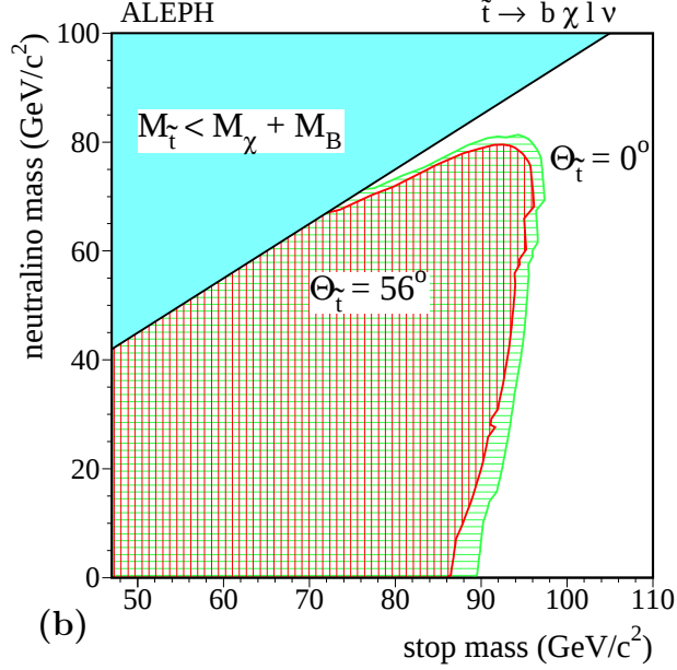
Figure 3: Excluded regions at 95% C.L. in the M_{\tilde{\chi}} vs M_{\tilde{t}} plane from \tilde{t} \rightarrow b \chi f \bar{f}' searches: (a) the W^* modes or (b) the leptonic modes are assumed to be dominant for the f \bar{f}' final states. The excluded regions are given for \theta_{\tilde{t}} = 0^\circ , corresponding to maximum \tilde{t} \tilde{t} Z coupling, and for \theta_{\tilde{t}} = 56^\circ , corresponding to vanishing \tilde{t} \tilde{t} Z coupling.
