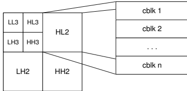
Fig. 3. Customized code-block dimensions.
