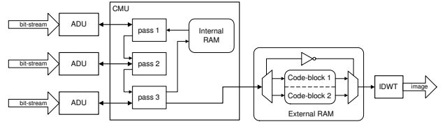
Fig. 5. Simplified view of the CMU architecture.
