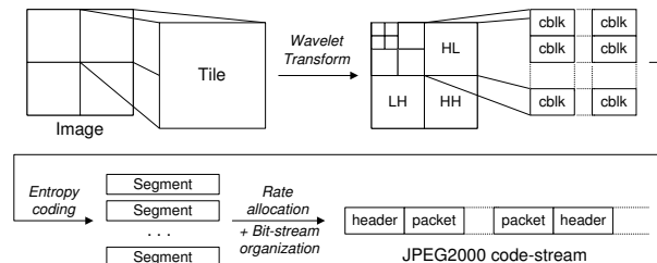
Fig. 1. Coding steps of the JPEG 2000 algorithm.
