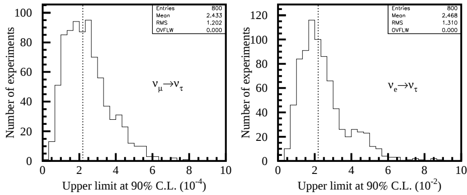
Fig. 6. Upper limits obtained at 90% C.L. [21], in absence of signal events, for 800 simulated experiments with the CHORUS expected background. The average value corresponds to the sensitivity to \nu_\mu \rightarrow \nu_\tau (left) and \nu_e \rightarrow \nu_\tau (right) appearance probability. The vertical line is the 90% C.L. upper limit obtained from the data.
