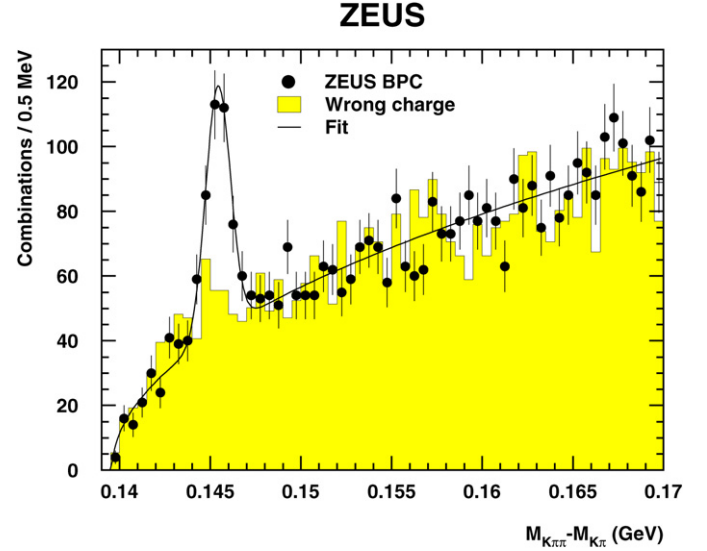
Fig. 1. The distribution of the mass difference, \Delta M = M(K\pi\pi_s) - M(K\pi) , for D^{*\pm} candidates with a measured scattered electron in the BPC. The histogram shows the \Delta M distribution for wrong charge combinations, normalised to the data in the region 0.151 < \Delta M < 0.167 . The normalisation factor is 1.07. The solid curve is the result of the fit described in the text.
