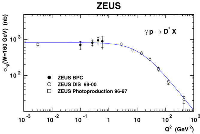
Fig. 4. The \gamma p cross section for D^{*\pm} production in the range 1.5 < p_T(D^*) < 9 GeV and |\eta(D^*)| < 1.5 as a function of Q^2 from this Letter (BPC), compared with previous results on D^* production in DIS [5] and photoproduction [7] for 1.5 < p_T(D^*) < 15 GeV and |\eta(D^*)| < 1.5 . The data are represented by points. The inner error bars are statistical while the open error bars are the sum of statistical and systematic uncertainties added in quadrature. The photoproduction point is drawn at Q^2 = 0.003 GeV 2 for convenience. The curve shows a fit to the data described in the text.
