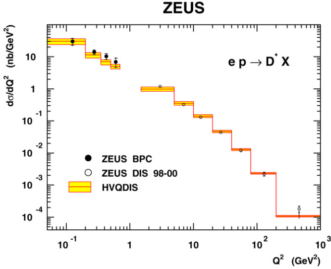
Fig. 3. The D^* production cross section as a function of Q^2 in the kinematic region 0.02 < y < 0.7 , 1.5 < p_T(D^*) < 9 GeV and |\eta(D^*)| < 1.5 for this measurement (BPC) and previous results on D^* production in DIS [5] (for 1.5 < p_T(D^*) < 15 GeV), compared to the HVQDIS NLO prediction. The data are represented by points. The inner error bars are statistical while the open error bars are the sum of statistical and systematic uncertainties added in quadrature. The shaded area indicates the theoretical uncertainties obtained by variations of the HVQDIS parameters.
