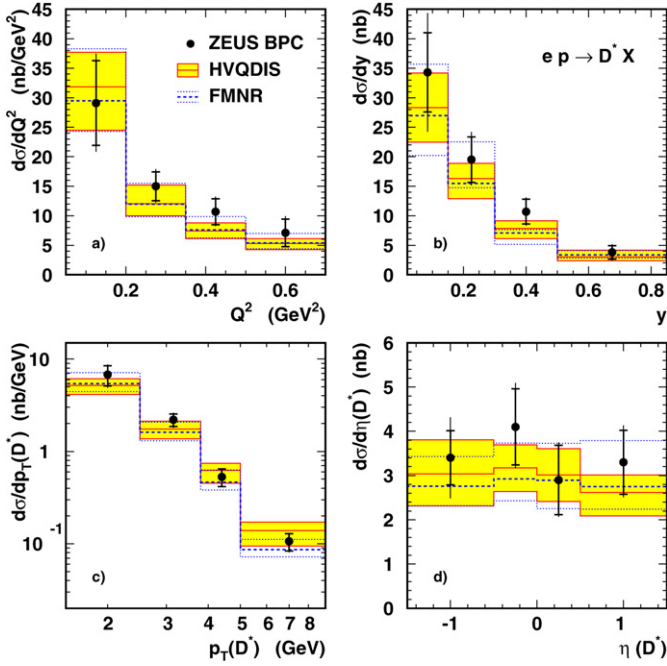
Fig. 2. Differential D^* production cross sections as a function of (a) Q^2 , (b) y , (c) p_T(D^*) and (d) \eta(D^*) compared to the HVQDIS and FMNR NLO predictions. Data are represented by points. The inner error bars are the statistical errors of the measurement while the open error bars are the sum of statistical and systematic uncertainties added in quadrature. The shaded area indicates the theoretical uncertainties obtained by variation of the HVQDIS parameters. The dashed and dotted lines represent the central value of the FMNR calculation and its uncertainty, respectively.
