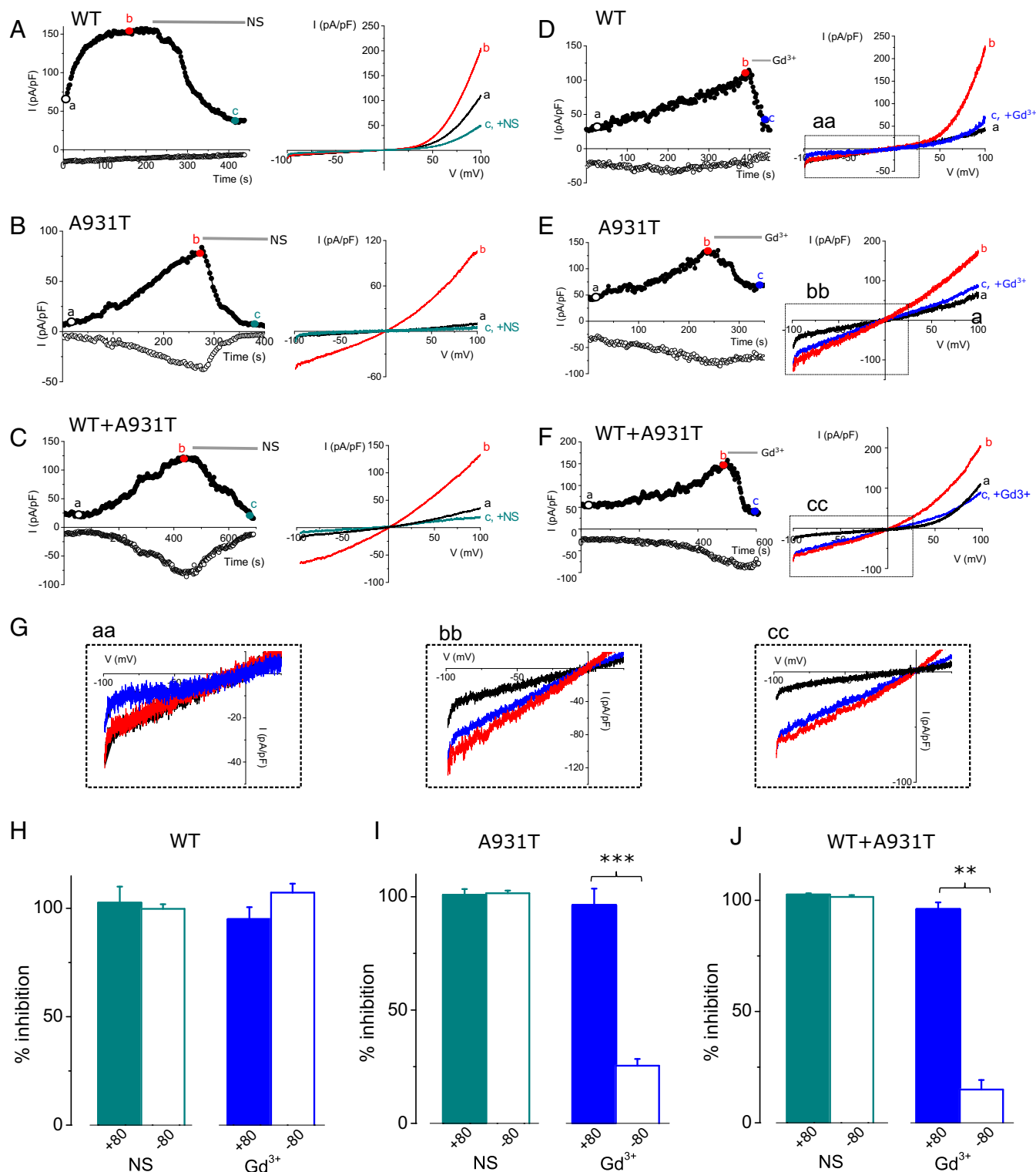
Fig. 2. A931T inward current is blocked by NS8395 but is less sensitive to Gd^{3+} . (A–C) Representative time courses (Left) and I–V traces (Right) of development of TRPM7 current for WT, A931T, and WT+A931T during application of TRPM7 antagonist NS8593 (NS, 10 \mu M). (D–F) Representative time courses (Left) and I–V traces (Right) of development of TRPM7 current for WT, A931T, and WT+A931T during application of Gd^{3+} (100 \mu M). (G) Enlarged view of inward currents (boxed area in A) in cells transfected with WT (aa), A931T (bb), and WT+A931T (cc) channels, in the absence and presence of Gd^{3+} . (H) Percentage inhibition of WT outward (+80 mV) and inward (–80 mV) currents upon application of NS8593 (green, n = 6 ) and Gd^{3+} (blue, n = 6 ). (I) Percentage inhibition of A931T outward (+80 mV) and inward (–80 mV) currents upon application of NS8593 (green, n = 8 ) and Gd^{3+} (blue, n = 5 ). (J) Percentage inhibition of WT+A931T outward (+80 mV) and inward (–80 mV) currents upon application of NS8593 (green, n = 6 ) and Gd^{3+} (blue, n = 6 ). Each column represents mean \pm SEM. *** P < 0.0001 , ** P < 0.001 (unpaired Student's t test).
