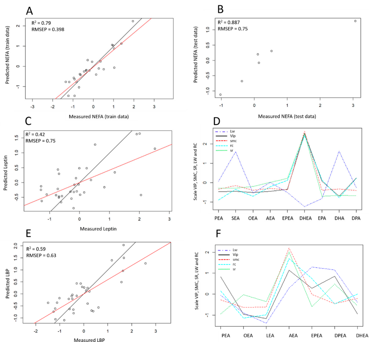
Figure 3. Modeling and validation of variable response according to a selected subset of the eCBome. ( A,B ) PLSR correlation plot between predicted and measured NEFA levels according to the selected eCBome mediator subset, illustrating the predictive quality of NEFA in the ( A ) training group ( n = 26 ) and ( B ) the test group ( n = 6 ). ( C ) PLSR correlation plot between predicted and measured leptin according to the selected eCBome mediator subset, constructed on all observations without cross-validation ( n = 32 ). ( D ) Scale plot illustrating the lw, rc, smc, sr and vip for each of the eCBome predictors in the variable-response prediction model. ( E ) PLSR correlation plot between predicted and measured LBP according to the selected eCBs mediator subset, construct on all observations without cross-validation ( n = 32 ). ( F ) Scale plot illustrating the lw, rc, smc, sr, and vip for each of the eCBs predictors in the variable-response prediction model. ( A,C,E ) The black line illustrated a perfect correlation ( R^2 = 1 ), the red line showed the measured correlation (five components for NEFA, four components for leptin, three components for LBP). ( D,F ) Color legend: red = smc (significance multivariate correlation); dark green = vip (variable importance in projections); light green = sr (selectivity ratio); dark blue = lw (loading weight); light blue = rc (regression coefficient). Abbreviations: see Table 1.
