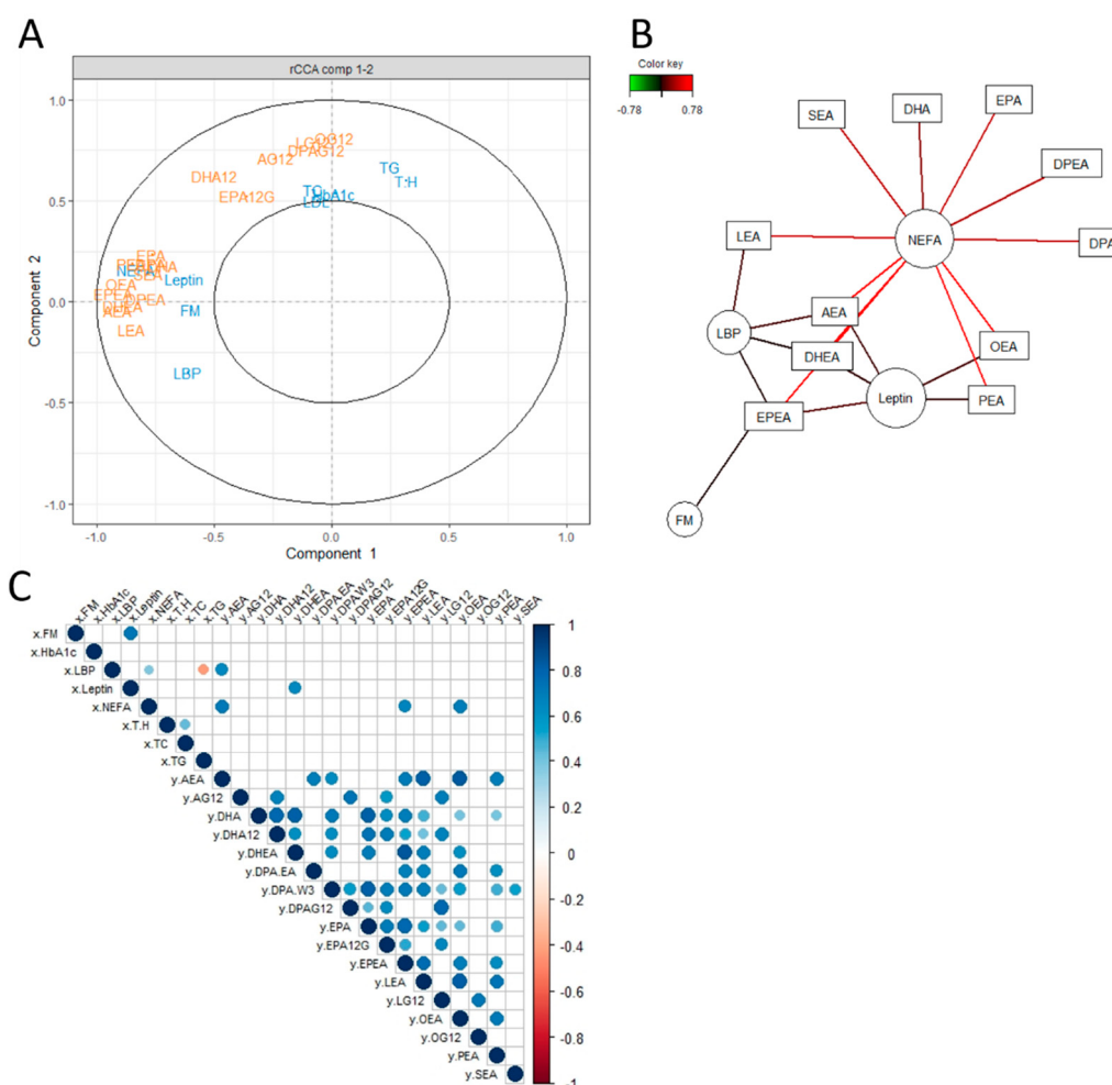
Figure 1. Unsupervised exploration of the relationship between measured eCB system-related mediators and biological parameters using regularized canonical correlation (rCCA) and correlation matrix. (A) Correlation circle plot allocating biological parameters and eCBome features along the main components derived from the integration of both data sets. The components correspond to the equiangular vector between x - and y -variates. The features in the area outside the inner concentric circle (radius < 0.5 ) were retained as significant and shown in the scatter plot. (B) Relevance network of top correlations between biological parameters (circles) and eCBome lipids (rectangles) with a cut-off = 0.55. Lines are colored according to the strength of the association score between two variables with red showing positive correlations. (C) Correlation matrix (Spearman with Holm's adjustment); positive correlations are displayed in blue and negative correlations in red color. The color intensity and the size of the circle are proportional to the correlation coefficients. "X" refers to the first data set, the metabolic biological parameters while "Y" refers to the second data set, the endocannabinoids. Abbreviations: see Table 1.
