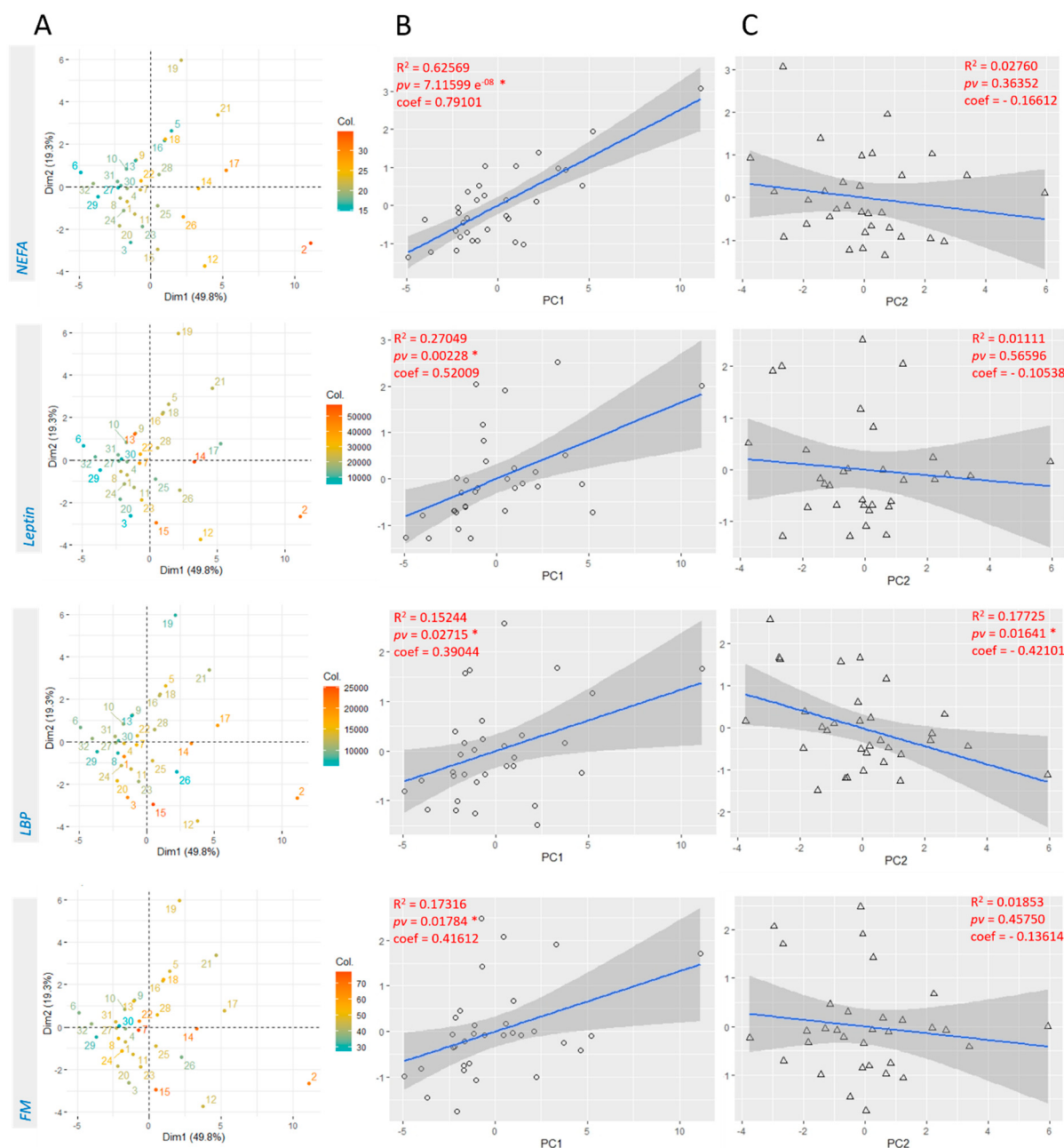
Figure 2. Deeper exploration of the relationship between measured eCB-related mediators and the biological parameters selected from rCCA using PCA. (A) Individual plots, the color gradient for each individual was established according to the concentration of the referred biological variable. (B) Scatterplots showing the linear relation between first principal components and the referred variable. (C) Scatterplots showing the linear relation between second principal components and the metabolic variable. The confidence interval is displayed in grey around the mean. (B,C) Each linear regression plot is accompanied by the R square, the p value and the coefficient of correlation (Pearson). Abbreviations: see Table 1.
