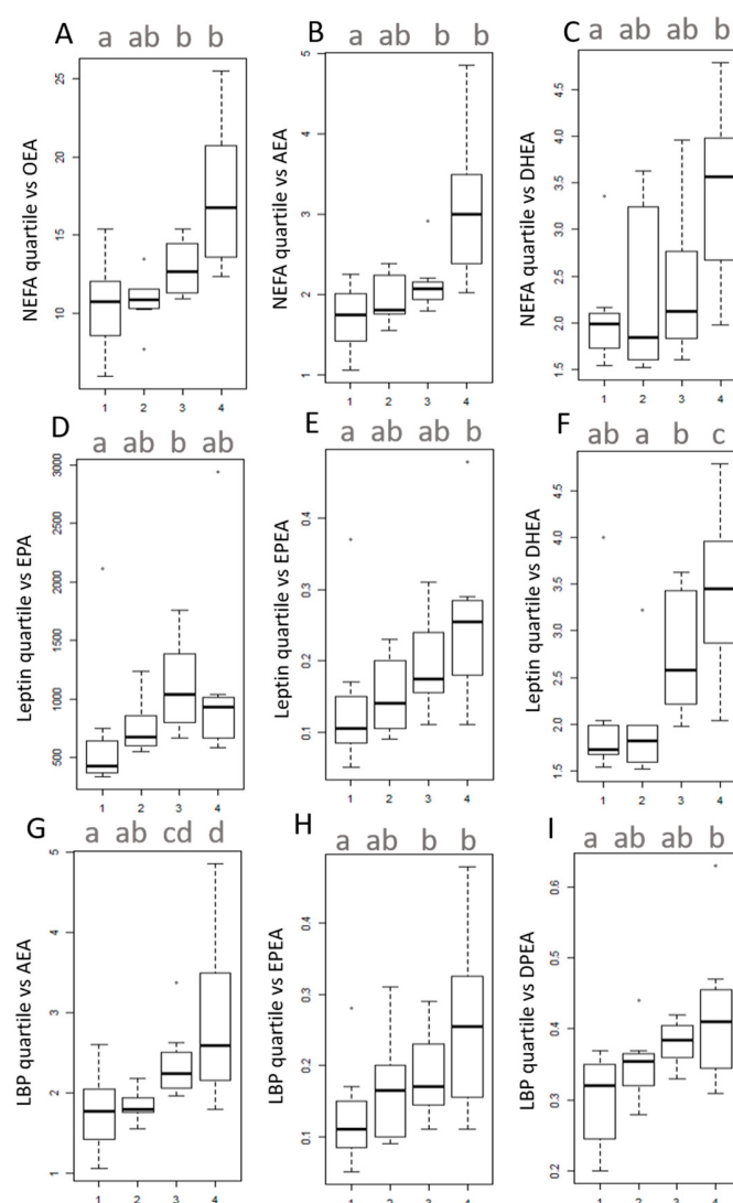
Figure 4. Univariate tests on quartiles. The number 1 corresponds to the lower quartile, while the number 4 corresponds to the upper quartile. (A,B) Boxplots of the concentration of (A) OEA, (B) AEA, (C) DHEA, according to NEFA quartiles. (D–F) Boxplots of the concentration of (D) EPA, (E) EPEA, (F) DHEA, according to leptin quartiles. (G–I) Boxplots of the concentration of (G) AEA, (H) EPEA, (I) DPEA, according to LBP quartiles. Data with different superscript letters are significantly different at p < 0.05 , according to the post-hoc ANOVA statistical analysis (C,F), or Kruskal–Wallis multiple comparisons test (A,B,D,E,G–I). Abbreviations: see Table 1.
