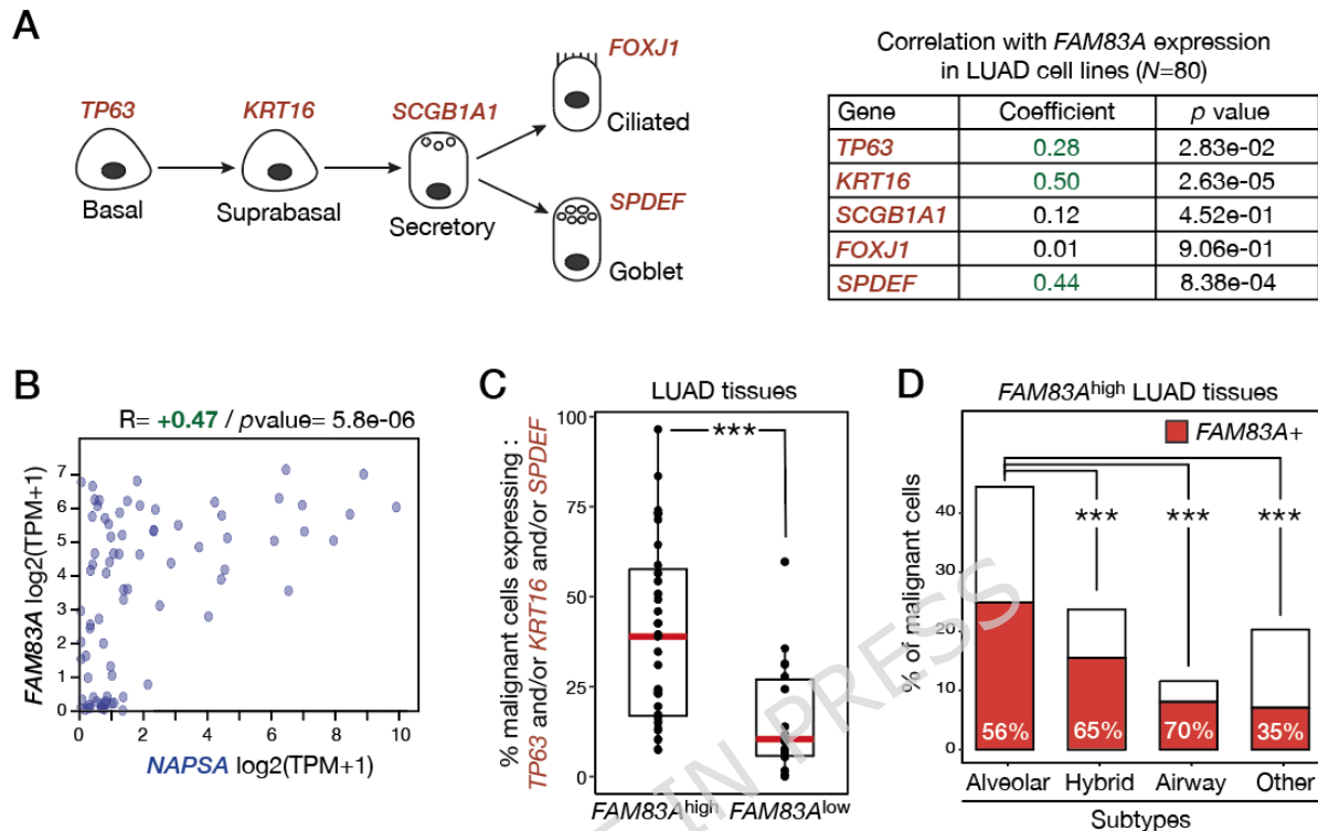
Fig. 4 FAM83A expression in LUAD coexists with AT2 marker NAPSA , and correlates with that of airway cell markers. (A) Indicated markers of lung airway cell subtypes were tested for their expression correlation scores (Spearman coefficient) with FAM83A in LUAD cell lines (CCLE), using the Depmap Portal. (B) Scatter plot showing co-expression of FAM83A and AT2-cell marker NAPSA in LUAD cell lines of the CCLE. (C) scRNA-Seq data of LUAD tissues were analyzed, and tumor samples were divided into FAM83A high ( \geq 30\% malignant cells expressing FAM83A ) and FAM83A low ( < 10\% malignant cells expressing FAM83A ) (t-tests; ***: p \leq 0.001 ). Boxplots represent the proportion of cells expressing at least one of the indicated markers in the different samples. (D) Malignant cells belonging to FAM83A high LUAD samples were classified into different subtypes (alveolar, hybrid, airway, other) according to the expression of specific markers (see text), and the proportion of cells expressing FAM83A was measured in each cell subtype (Chi-square test; ***: p \leq 0.001 )
