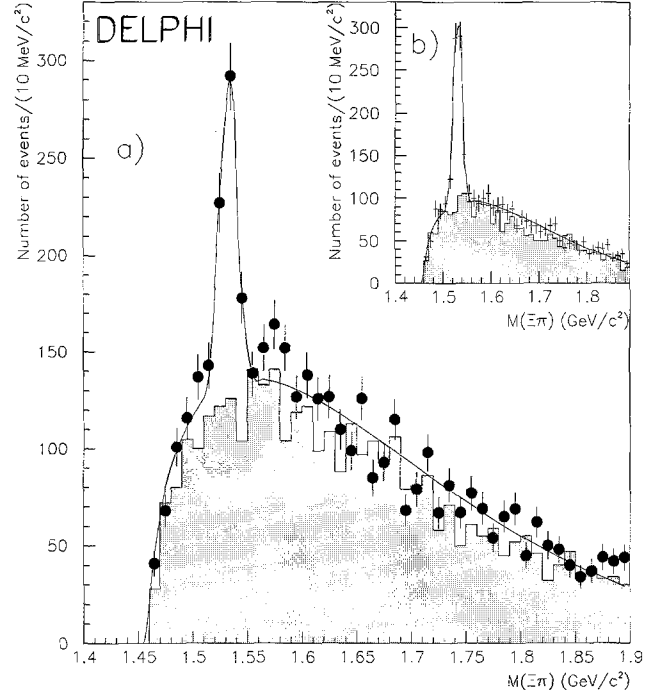
Fig. 3. a) \Xi^-\pi^+ ( \Xi^+\pi^- ) invariant mass distribution. The shaded histogram represents the invariant mass spectrum of the wrong sign combinations. b) The same mass distribution as in a) produced with simulated events
