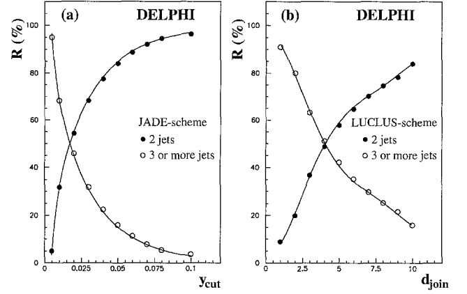
Fig. 7. The jet multiplicities found by JADE and LUCCLUS recombination schemes as a function of the jet resolution parameter. The solid lines represent the JETSET prediction
