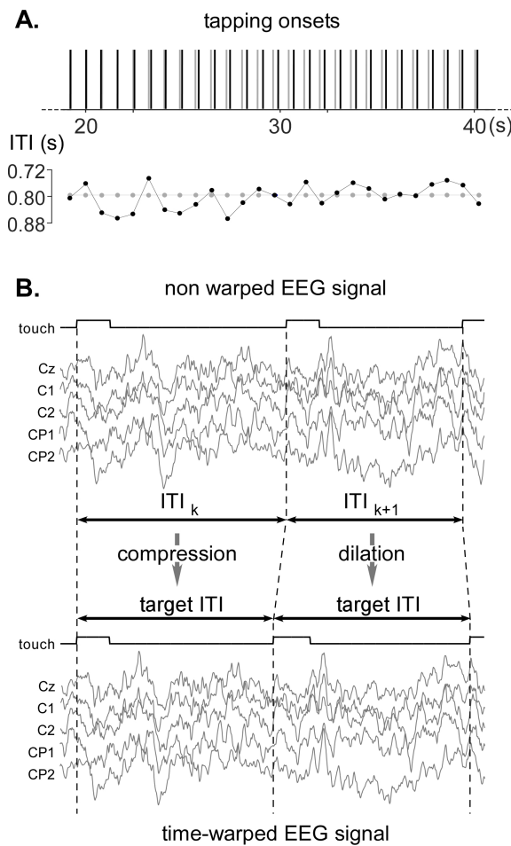
Figure 4. EEG time-warping procedure. A. As shown in this representative trial of the finger-tapping to the beat task, the inter-tap interval (ITI) fluctuated from tap to tap, with a mean ITI of 800 ms. B. The time-warping procedure consists in compressing or dilating the EEG signals recorded within each ITI such as to scale it to a fixed target ITI of 800 ms. The compression and dilation of the EEG segments was computed by linear interpolation of the non-time-warped signals.
