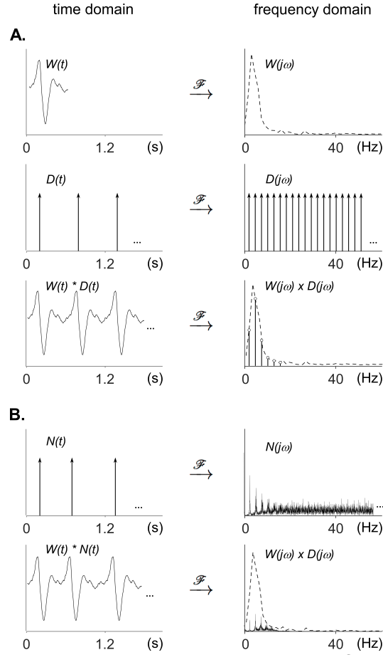
Figure 1. Time and frequency domain representation of periodic and non-strictly-periodic signals. A. Time domain and frequency domain representations of a unitary waveform W(t) , a periodic train of impulses (Dirac comb; D(t) ), and a periodic signal corresponding to the convolution of W(t) and D(t) in the time domain, and the multiplication of W(j\omega) and D(j\omega) in the frequency domain. Note that the Fourier transform of the periodic signal has a spectrum that concentrates on the fundamental frequency and harmonics determined by the periodicity of the Dirac comb, with a relative amplitude distribution that is determined by the shape of the spectrum of the unitary waveform. B. Time domain and frequency domain representations of a non-strictly-periodic signal corresponding to the convolution of W(t) with a non-strictly-periodic train of impulses N(t) . In contrast to the spectrum of the strictly-periodic Dirac comb D(j\omega) , the frequency spectrum of the non-strictly-periodic train of impulses N(j\omega) is not constituted of isolated peaks at the fundamental frequency and harmonics. Instead, the energy of the signal spreads to surrounding frequencies, and the spectrum will become more and more random if the non-periodicity is increased. The spectrum of the non-strictly-periodic signal obtained by multiplying the spectrum W(j\omega) of the unitary waveform with the spectrum N(j\omega) of the non-strictly-periodic train of impulses, contains peaks having a lower amplitude as compared to the strictly-periodic signal.
