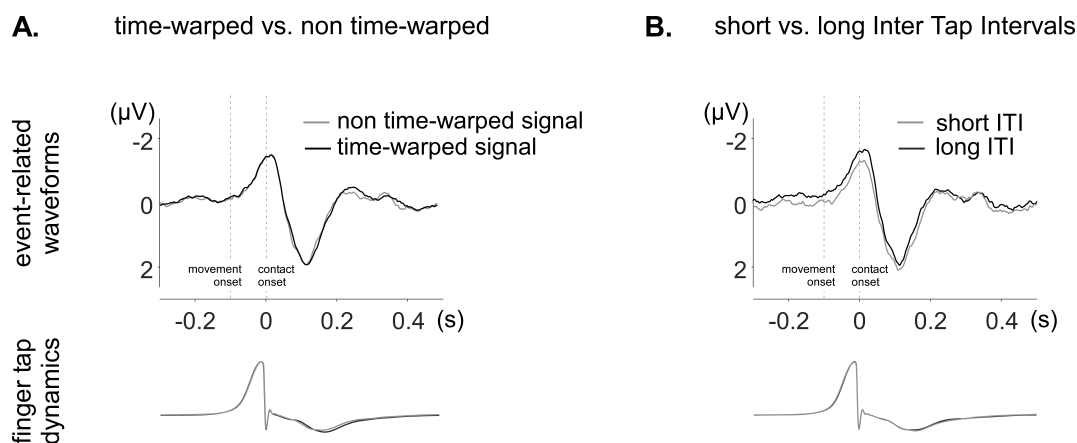
Figure 7. Time-domain analysis of the unitary EEG waveforms obtained in the tapping alone condition. The average waveforms (electrode Cz) were obtained by aligning EEG segments to the onsets of the contact of the fingertip with the table. The finger tap dynamics recorded by the movement sensor are shown in the lower part of the figure, also averaged relative to contact onset. A. Average waveform of the non-time-warped EEG signal (grey) and the time-warped EEG signal (black). In both non-time-warped and time-warped signals, a clear EEG response is observed, time-locked to the contact onset, and consisting of a negative peak concomitant to the tapping, followed by a positive peak maximal approximately 110 ms after tapping. The non-time-warped and time-warped waveforms are highly similar, except for a slight smoothing of rapid activities in the time-warped signal. B. Waveforms obtained by averaging EEG segments separately for short ITIs (grey) and long ITIs (black). The period preceding contact onset was more negative for long ITIs as compared to short ITIs. Furthermore, the negative peak concomitant to the finger contact was broader.
