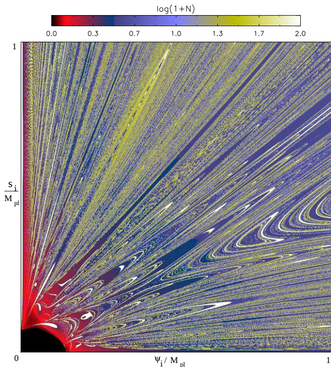
FIG. 13: Mean number of e-folds (truncated at 100) obtained from 512^2 initial field values (\psi_i/M_{\text{pl}}, s_i/M_{\text{pl}}) for the SUGRA F-term model. The initial field velocities are assumed to vanish and the potential parameter is fixed at M = 10^{-2}m_{\text{pl}} . As for the original hybrid model, the mean is computed from 2048^2 trajectories (see Fig. 1). The set of initial field values producing enough inflation is again of dimension two with a fractal boundary.
