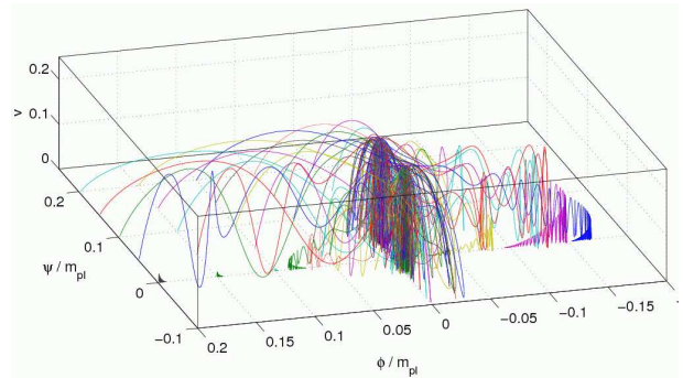
FIG. 2: Phase space v^2(\phi, \psi) for 25 trajectories and vanishing initial velocities. The potential parameters are fixed to the values M = 0.03m_{\text{pl}}, \mu = 636m_{\text{pl}}, \nu = 6.36 \times 10^{-4} . All trajectories end on the three attractor of the dynamical system: the two global minima of the potential, and the inflationary valley with almost vanishing slow-roll velocity. These three attractors induce the chaotic behavior.
