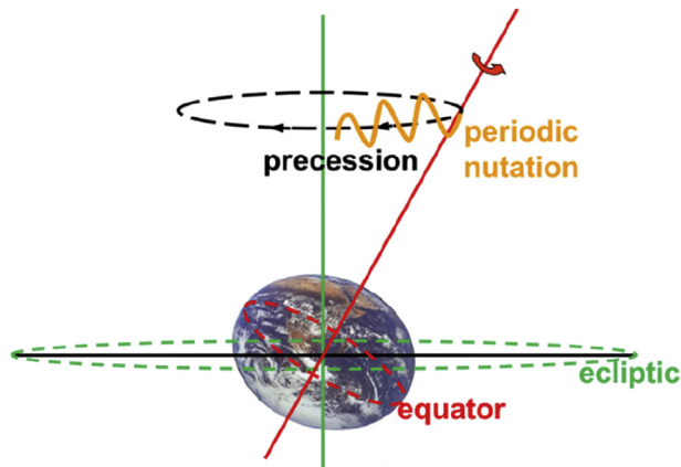
Fig. 1. Representation of precession and nutation of the Earth.
