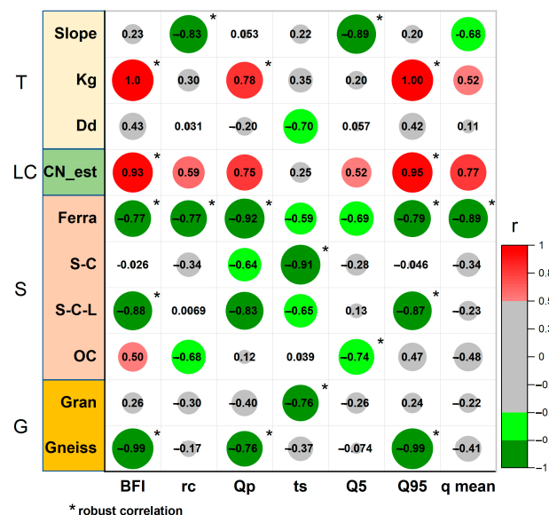
Figure 11. Correlation plot between HSs and CDs using Pearson’s coefficient r . The catchment descriptors are color-coded according to their generic group: topography (T), land cover (LC), soil (S), and geology (G). The size of the circles indicates the strength of the correlation, with red corresponding to positive and green to negative correlations. Gray circles mean poor correlation ( r < |0.5| ). ‘*’ indicates a robust correlation.
