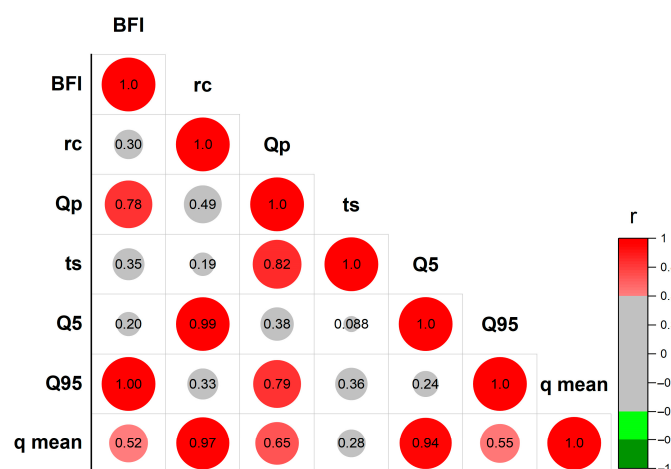
Figure 10. Correlation plot between hydrological signatures using Pearson's coefficient r . The size of the circles indicates the strength of the correlation, with red corresponding to positive and green to negative correlations. Gray circles mean poor correlation ( r < |0.5| ).
