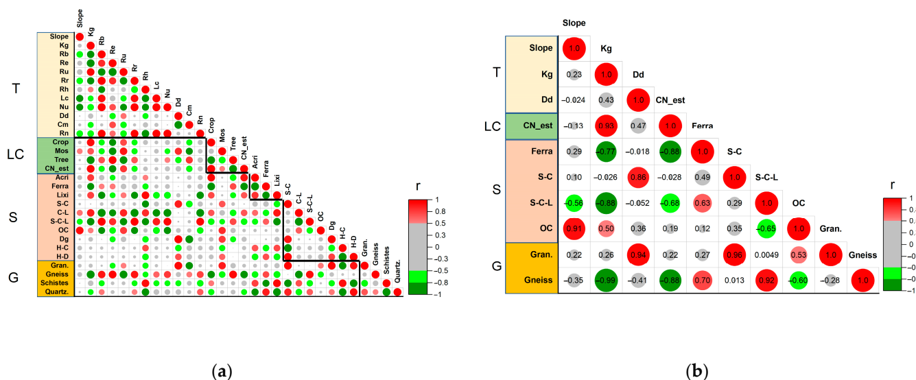
Figure 5. Correlation plot between (a) all catchment descriptors, and (b) selected catchment descriptors, based on Pearson's coefficient r . The catchment descriptors are color-coded according to their generic group: topographic (T), land cover (LC), soil (S), and geology (G). The size of the circles indicates the strength of the correlation, with red corresponding to positive and green to negative correlations. Gray circles mean poor correlation ( r < |0.5| ).
