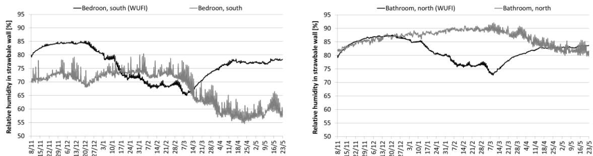
Figure 8 (left) relative humidity under bracing panel of south wall in the bedroom in Uccle, simulated with WUFI Plus software (right) relative humidity under bracing panel of north wall in the bathroom in Uccle, simulated with WUFI Plus software.
