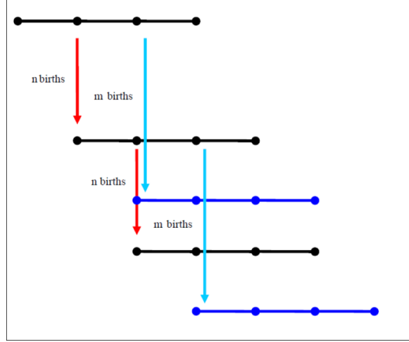
Figure 5: The lifecycle fertility model.
