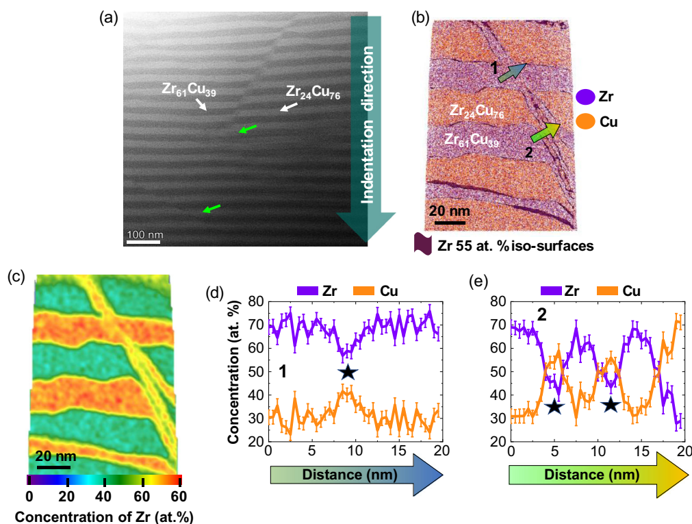
Figure 3. Chemical evolution along shear banding process underneath a nanoindent on a 3 \mu\text{m} thick NL with \Delta = 50 nm. a) The HAADF-STEM image shows the propagation of the SB which stops at the stiffer \text{Zr}_{24}\text{Cu}_{76} layers (green arrows), acting as deformation barriers. b) APT sample highlighting the severe deformation along SB events causing a mismatch of the original layer stack (5 nm thin slice viewed along the x axis, extracted from Figure 1e. c) The 2D contour plot of Zr (identical region with (b)) and d,e) 1D concentration profiles (i.e., within cylindrical regions of interest of \Phi 4 \times 20 nm) of two different points across the SB path indicated by (1) and (2) gradients in (b) highlighting the large chemical intermixing between the layers.
