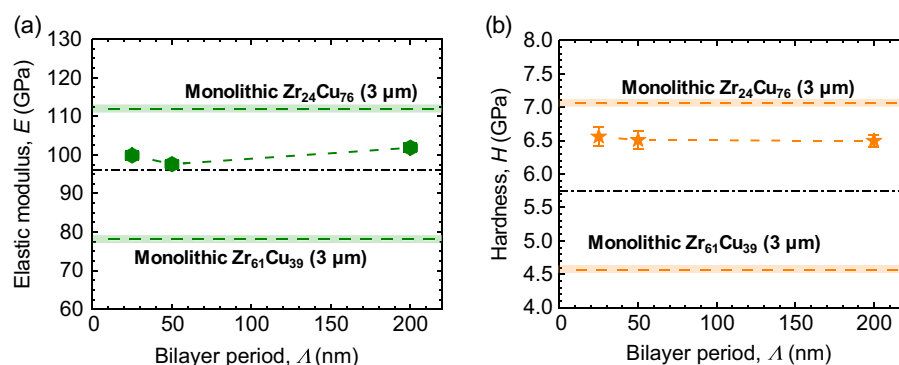
Figure 2. Comparison between a) elastic modulus ( E ) and b) hardness ( H ) values from CSM nanoindentation for 3 \mu\text{m} thick NLs as a function of bilayer period ( \Delta ). The values of E remain close to the rule of mixture (ROM) (i.e., black dash-dot lines), while the values of H are higher and close to those of the harder \text{Zr}_{24}\text{Cu}_{76} . The dashed lines in the graphs represent the values for monolithic reference films ( \text{Zr}_{24}\text{Cu}_{76} and \text{Zr}_{61}\text{Cu}_{39} ) and the shadowed regions represent the respective error bars.
