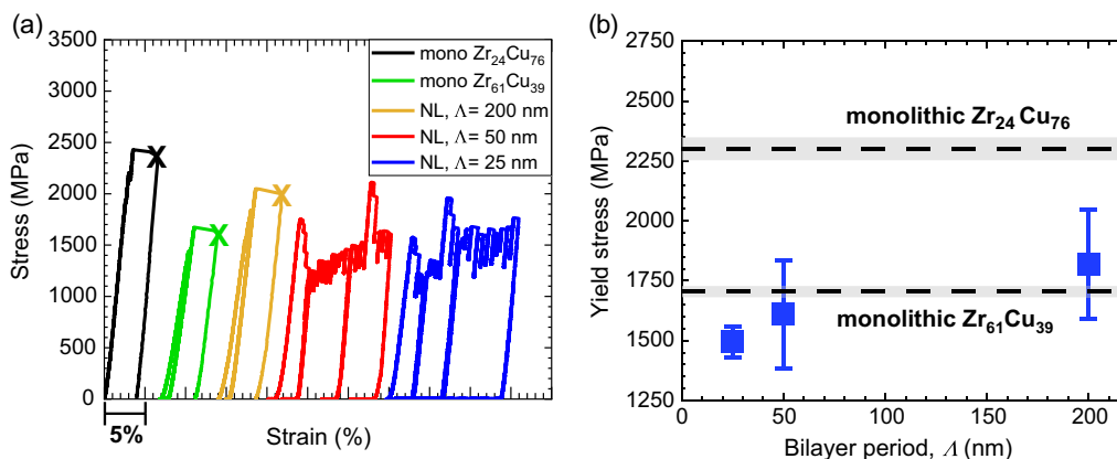
Figure 4. a) Selection of micropillar compression curves for 3 μm thick monolithic films and NLs (the rest of the curves are reported in Figure S6, Supporting Information). The curves have been shifted horizontally to facilitate data visualization. Monolithic films and NLs with \Lambda = 200 nm fail with formation of large SB events which cause strain bursts and load drops to zero; for NL with \Lambda = 50 and 25 nm, SBs propagation is suppressed while reporting a large apparent plasticity (the load drops are due to the two unloading cycles performed during the tests). b) Evolution of the yield stress ( \sigma_y ).
