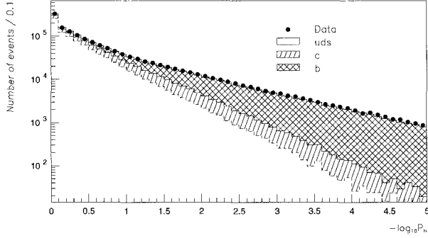
Fig. 3. Distribution of -\log_{10}(P_H) for the data and for different flavour contributions in the simulation corrected to have the same resolution as the data
