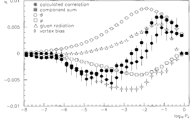
Fig. 4. Total hemisphere correlation and individual contributions as a function of the cut value \log_{10} P_H
