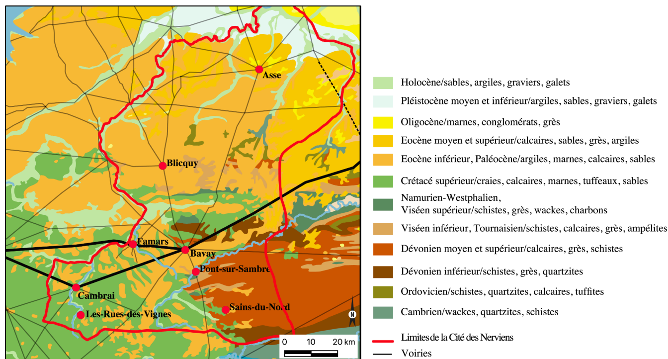
Fig. 6. Simplified geological map of the Civitas Nerviorum, modified after BGRM ( http://sigesnpc.bgrm.fr/Geologie-en-Nord-Pas-de-Calais.html ). © Raphael Clotuche and Laurent Deschodt, Inrap.
