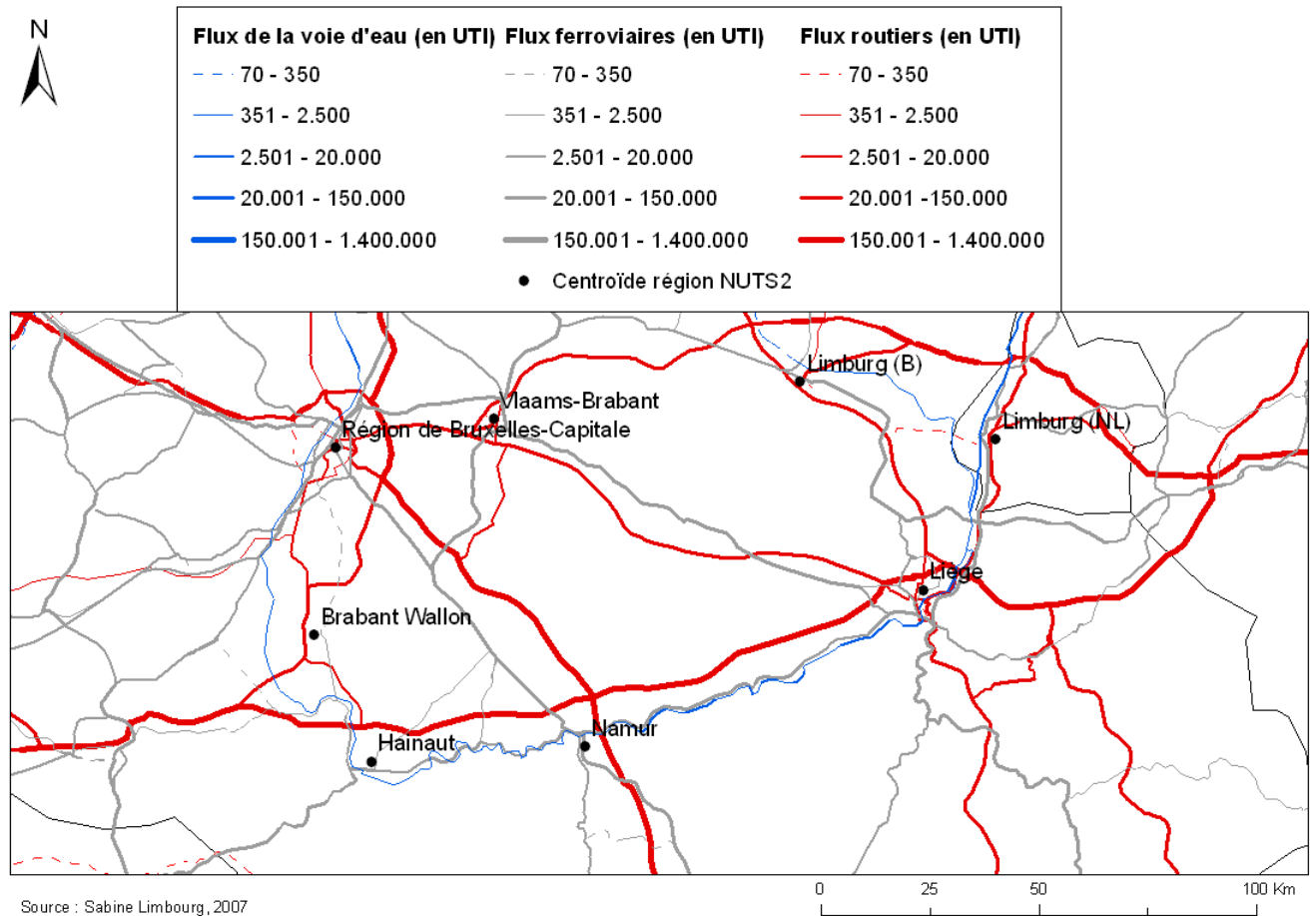
Figure 5.15. Affectation multi-flux et multimodale - Wallonie.
