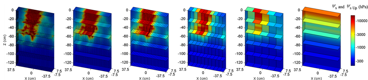
Fig. 4. Discretisations of the maize crop soil domain used for the first simplifying approach. The colour scale gives the soil water potential distribution at the end of the high-transpiration-rate scenario on silt loam.
