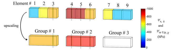
Fig. 1. Examples of the relation between \psi_{s,k} and \psi_{\text{sr Up},g} . Cubes are soil elements whose SWP, \psi_{s,k} , is represented by the colour scale. Parallelepipeds are groups of three, upscaled, soil elements, whose upscaled soil–root interface water potential \psi_{\text{sr Up},g} is represented by the same colour scale. Green vertical lines, in elements 3–6 and groups 1 and 2, are root segments.
