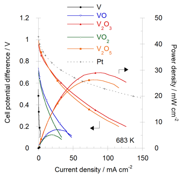
Figure 4. (color online) Operational curves for the thin film solid oxide fuel cell with vanadium oxide anodes with different as-deposited stoichiometries at 683 K. The performance of a comparable cell with porous Pt anode fuel cell is included for comparison.
