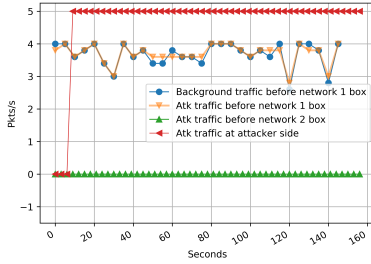
Figure 5: Reflection attack
