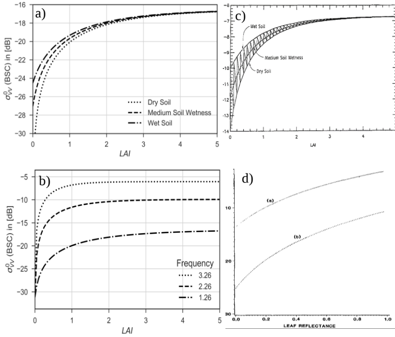
Fig. 1: \sigma^0 (BSC) versus LAI as calculated from RO-M for a) three different soil wetness conditions at frequency 1.26 GHz: 0.25 (wet), 0.15 (medium), 0.05 (dry), for b) three different acquisition frequencies in GHz: 3.26, 2.26, 1.26, for c) BSC versus LAI for a corn canopy from [1], microwave frequency at 17.0 GHz, VV polarization, angle of incidence = 50° wetness conditions: 0.25 (wet), 0.15 (medium), 0.05 (dry), for d) Backscattering coefficient versus leaf reflectance from [2] to simulate frequency dependence of backscattering coefficient. Leaf angles are assumed to be uniformly distributed with an average angle of 45°. LAI = 2.0, Soil reflectance = 0.2. Angle of incidence: (a) 20°; (b) 50°.
