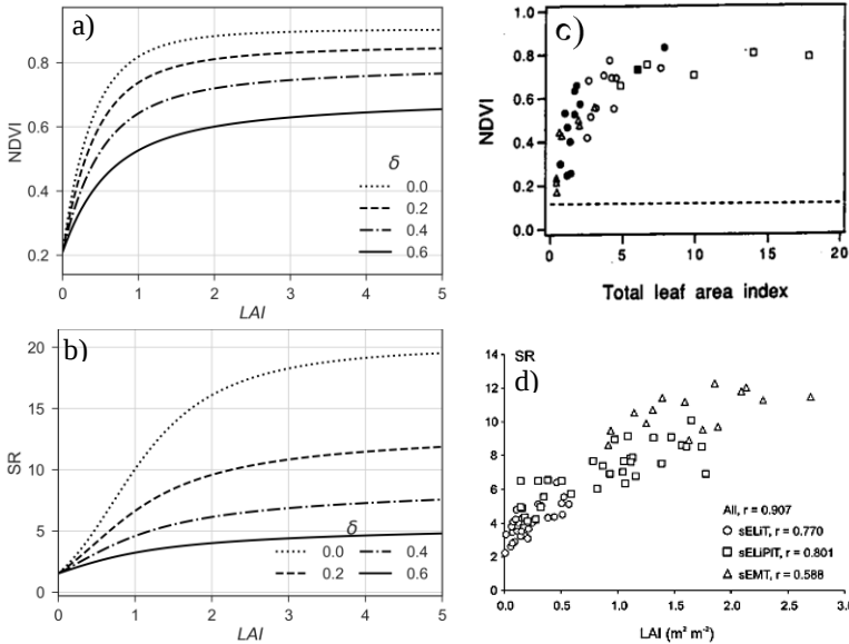
Fig. 2: NDVI and NIR-Red-Ratio (SR) versus LAI for a) and b) at different weighting parameter \delta for dominance of geometric or shadowed surface over volumetric volume scattering as calculated from RO-M. Acquisition Scenario: Leaf angle = 45^\circ , angle of incidence = 50^\circ , scattering angle = 30^\circ , relative azimuth angle = 50^\circ . Band ratios calculated with PROSPECT model. Leaf structure parameter = 1. Chlorophyll a+b content = 20. Carotenoids content = 3. Brown pigments content = 0.40. Equivalent water thickness = 0.0005. Dry matter content = 0.0085. For c) relationship between NDVI and LAI for three different California vegetation types at two different seasons from [3] and for d) relationship between LAI and ASTER SR for different mountain birch forest types from [1].
