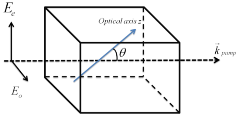
Figure 3-3 An uniaxial birefringent crystal. The principal plane of the crystal is the plane of the wave vector k and the optical axis of the crystal. An ordinary polarized wave has a polarization perpendicular to this plane and an extraordinary polarized wave has polarization in the principal plane.
