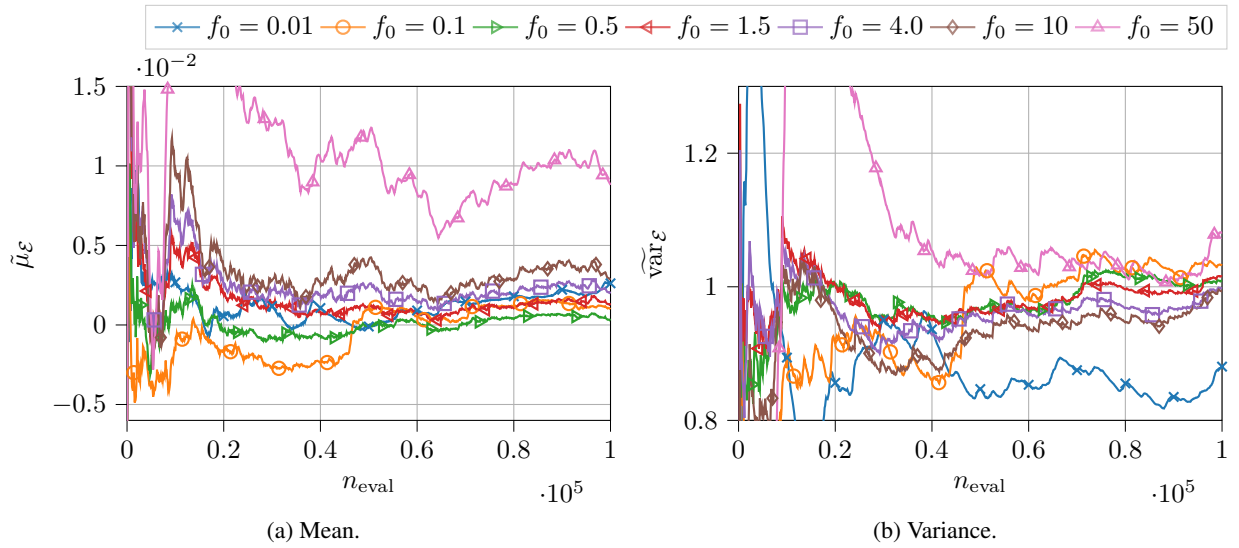
FIG. 17: Comparison of the convergence of the mean (a) and variance (b) of \mathcal{E} as a function of the number of model evaluations for the ISDE algorithm for different value of f_0 .
