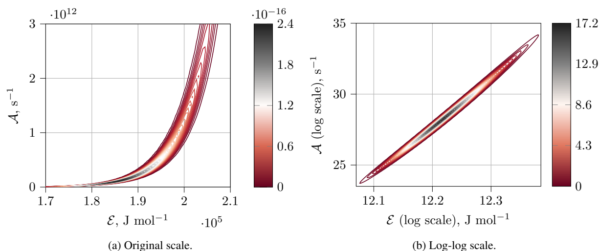
FIG. 4: Bivariate posterior densities for the parameters \mathcal{A} and \mathcal{E} in the original parameter space (left) and logarithmic scales (right). Fourteen density contours are shown with intensity represented on the colorbars on the right of each plot.
