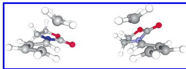
FIGURE 2. Structure and relative energy (B3LYP 6-31G**) of two relevant transition states for cycloaddition of ethylene and N -dienyloxazolidin-2-one: (left) TS_{anti} , 0 kcal·mol -1 , dihedral angle C(=O)-N-C(1)-C(2) = 168.1^\circ ; (right) TS_{syn} , 2.79 kcal·mol -1 , dihedral angle C(=O)-N-C(1)-C(2) = 39.5^\circ . Key: gray, C; white, H; red, O; blue, N.
