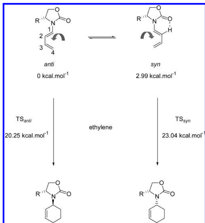
FIGURE 1. Relative energies (B3LYP/6-31**) of anti and syn conformers of the N -(butadienyl)oxazolidin-2-one ( R = H ) and the transition states of their reaction with ethylene (energy of both transition states is relative to the sum of the reactants energies considering the diene in its anti conformation).
