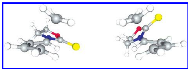
FIGURE 3. Structure and relative energy (B3LYP 6-31G**) of two relevant transition states for cycloaddition of ethylene and N -dienyloxazolidin-2-thione: (left) TS anti , 0 kcal·mol -1 , dihedral angle C(=S)–N–C(1)–C(2) = 164.2°; (right) TS syn , 4.60 kcal·mol -1 , dihedral angle C(=S)–N–C(1)–C(2) = 44.6°. Key: gray, C; white, H; red, O; blue, N; yellow, S.
