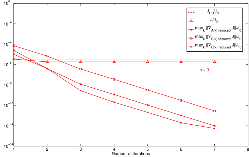
Figure 1: Convergence of \mathcal{J} and its gradients for third order approximation, normalized by \mathcal{J}_0 the \mathcal{H}_2 norm of the initial model
