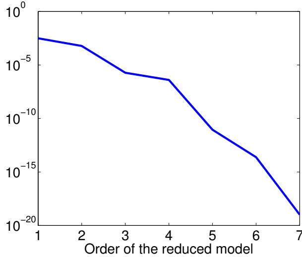
Figure 2: Convergence of \mathcal{J} for reduced model of order n = 1 to 7, normalized by \mathcal{J}_0 the \mathcal{H}_2 norm of the initial model
