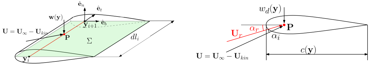
Figure 4: Left: Wing element between two wing profiles, and identifying a plane \Sigma containing the lifting line. Right: Cross section containing the chord point \mathbf{P} where the velocities are applied.
