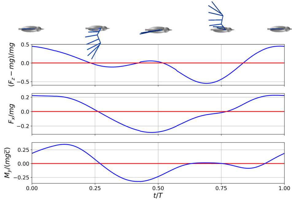
Figure 12: Dimensionless forces and pitching moment developed by the flier, expressed in the fixed frame O(X, Z) .
