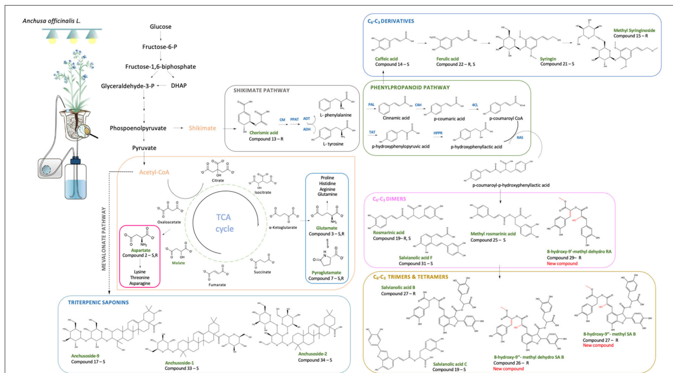
FIGURE 6 | Schematic representation of the main PMs and SMs influenced by the AMF-plant symbiosis in relation to different biosynthetic pathways. Upregulated compounds are reported in green accompanied by the letters R and/or S, indicating whether they were found upregulated in roots and/or shoots, respectively (CM, chorismate mutase; PPAT, prephenate aminotransferase; ADT, arogenate dehydratase; ADH, arogenate dehydrogenase; PAL, phenylalanine ammonia-lyase; TAT, tyrosine aminotransferase; C4H, cinnamic acid 4-hydroxylase; HPPR, hydroxyphenylpyruvate reductase; 4CL, 4-coumaric acid coenzyme A-ligase; RAS, rosmarinic acid synthase; HXL, hydroxylase).
