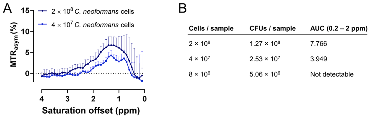
Fig. 2. CEST imaging of Cryptococcus cell phantoms. C. neoformans cells were suspended in PBS, counted and afterwards plated for colony-forming unit (CFU) counting. A) MTR_{asym} curves and B) quantification of the area under the curve (AUC, from 0.2 to 2 ppm) for different cell densities.
