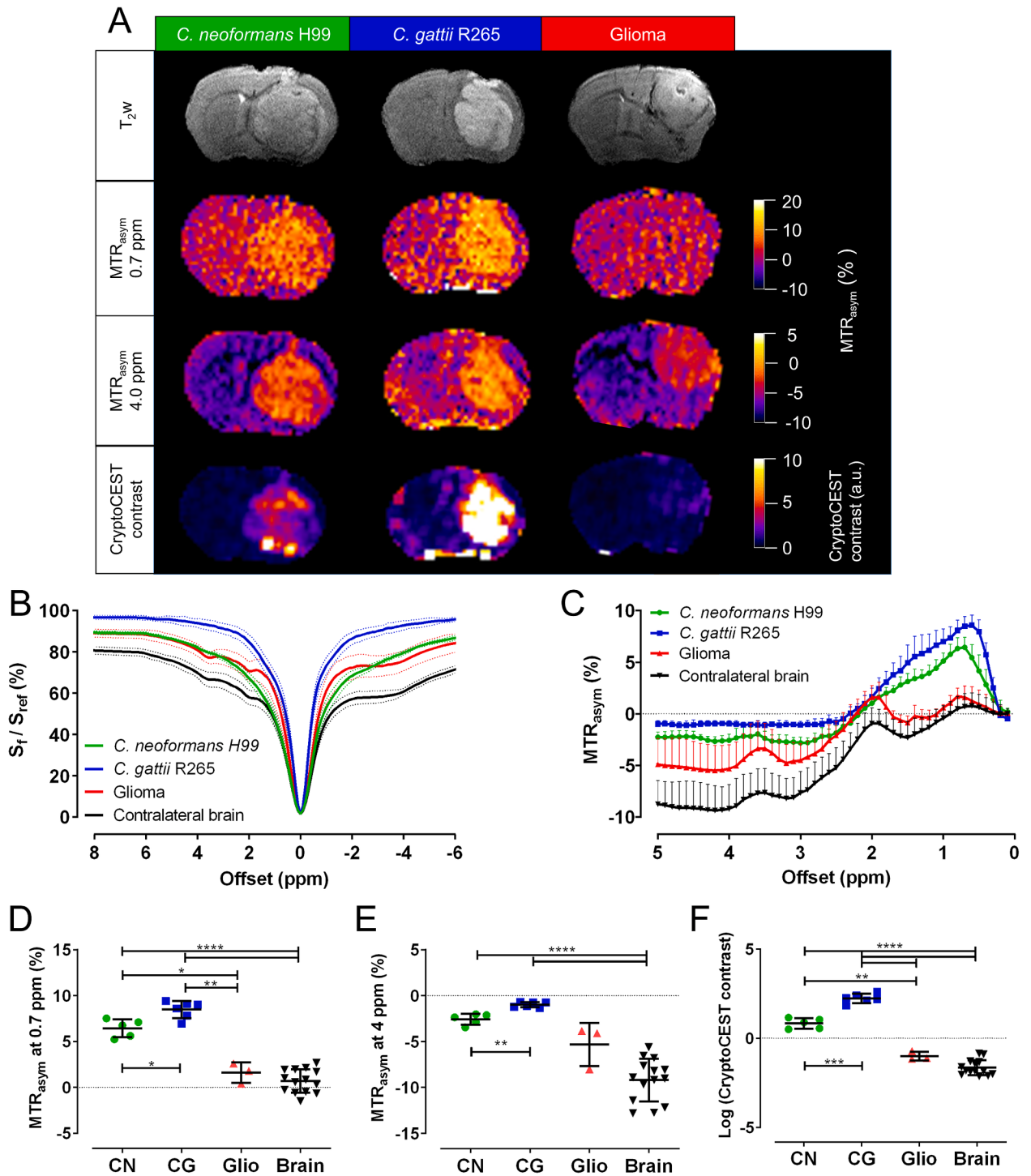
Fig. 5. CEST imaging of mice with cryptococcomas and gliomas. Mice were injected intracranially with C. neoformans (H99) cells ( n = 5 ), C. gattii (R265) cells ( n = 6 ) or neurospheres-cultured CT-2A cells ( n = 3 ). CEST images were acquired 8 days (cryptococcoma) or 14 days after inoculation (glioma). A) T_2 -weighted anatomical MRIs, MTR_{asym} maps at 0.7 and 4 ppm, and CryptoCEST maps for representative animals. B) Z-spectra. C) MTR_{asym} curves. D-F) Quantification of the MTR_{asym} contrast at 0.7 ppm (D), at 4 ppm (E) and logarithm of the CryptoCEST contrast (F) for C. neoformans (CN) and C. gattii (CG) cryptococcomas, gliomas (Glio) and the contralateral brain tissue (Brain). All graphs show individual values and/or mean \pm SD per group, Welch's ANOVA with Dunnett's T3 post-test. *: p < 0.05 , **: p < 0.01 , ***: p < 0.001 , ****: p < 0.0001 .
