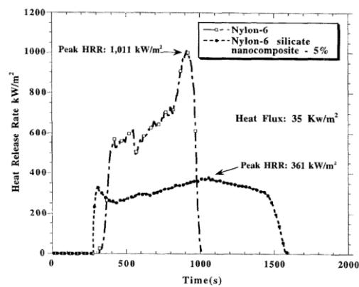
Figure 1.13: Comparison of the Heat Release Rate (HRR) plot for nylon-6 silicate- nanocomposite (mass fraction 5%) at 35kW/m² heat flux, showing a 63% reduction in HRR for the nanocomposite [150].
