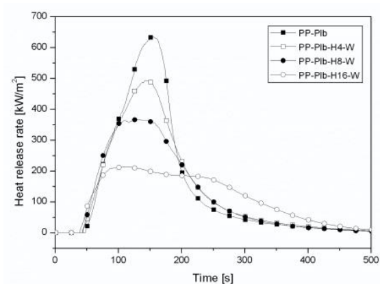
Figure 1.14: Heat release rate curves as a function of HNTs (H) loading for reference and PP/HNTs nanocomposites prepared by water-assisted extrusion (W) with PP-g-MA (Plb) [30].
