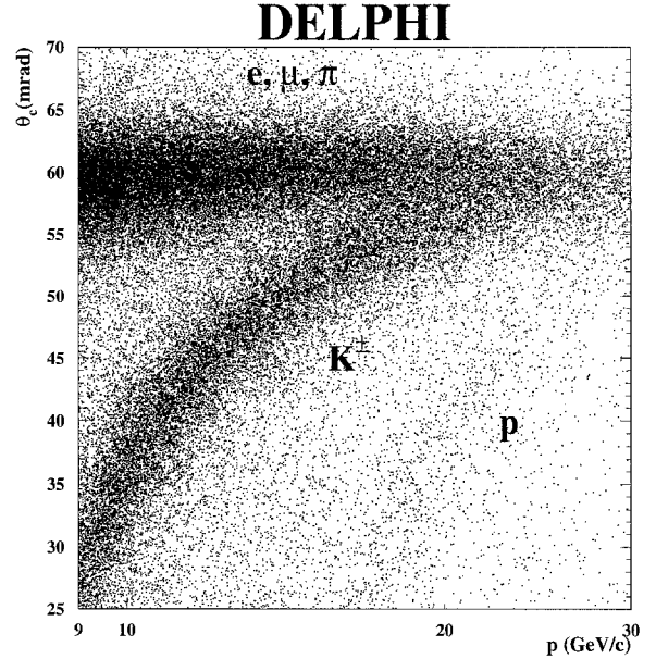
Fig. 2. Mean Cherenkov angle versus particle momentum
