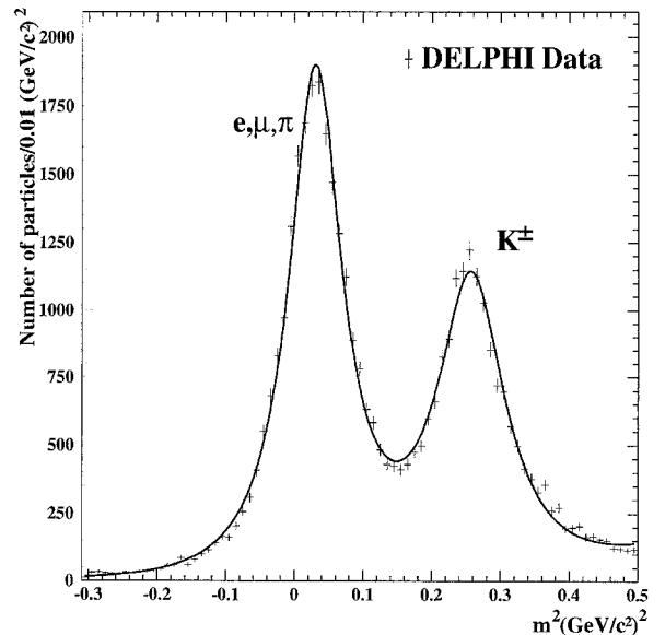
Fig. 3. Mass squared distribution using the RICH detector for all charged particles with 10 < p < 18 GeV/c. The curve shows the fit of two Breit-Wigner distributions
