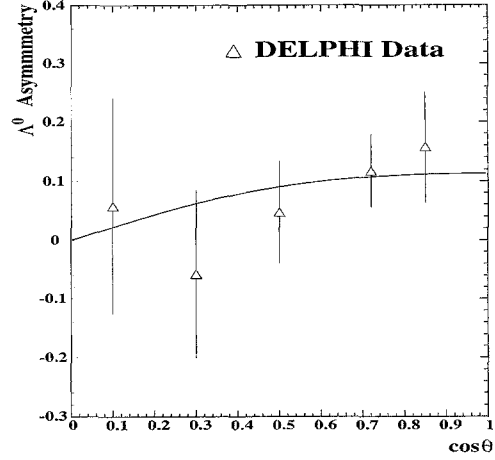
Fig. 8. \Lambda^0 asymmetry as a function of the cosine of the polar angle \theta . Equation (3) has been fitted to these data (curve)
