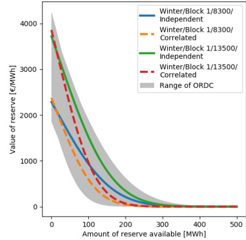
Fig. 1. Example of ORDCs under different variants.
