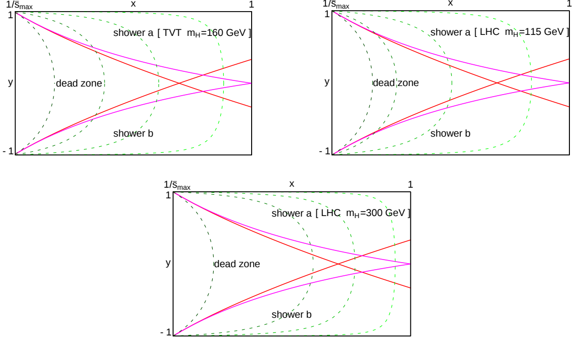
Figure 8: Radiative phase space in the x, y plane, as in Fig. 7 but with contours corresponding to constant values of p_T superimposed in green, from lightest to darkest (right to left) respectively these are, p_T = 10 GeV, p_T = 40 GeV, p_T = 80 GeV and p_T = m_H . The region into which the two shower progenitors cannot emit radiation is again marked ‘dead zone’; for HERWIG this area is bounded in red while for Herwig++ it lies between the magenta lines. The three plots correspond to the three scenarios under study in the remainder of the paper: a Higgs boson of mass 160 GeV at the Tevatron, a Higgs boson of mass of 115 GeV at the LHC, and a Higgs boson of mass 300 GeV also at the LHC. The area with emissions p_T > m_H is entirely within the dead zone in all scenarios.
