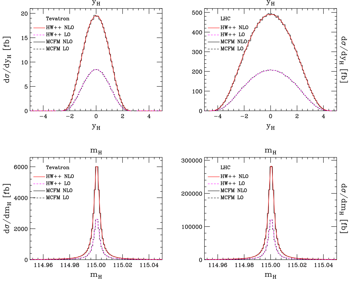
Figure 1: Comparisons of the POWHEG implementation in Herwig++ and the NLO parton level code MCFM [47], for the Higgs boson rapidity ( y_H ) and mass ( m_H ) distributions in the process g g \rightarrow H \rightarrow \tau^+ \tau^- . Results on the left are obtained for p\bar{p} collisions at the Tevatron ( \sqrt{s} = 1.96 TeV) while those on the right are for LHC pp collisions ( \sqrt{s} = 14 TeV).
