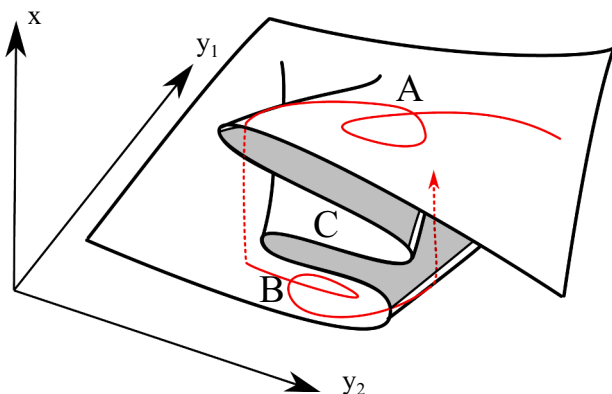
Fig. 12. Schematic diagram showing fast-slow dynamics in phase space: x represents a fast variable and y_1, y_2 slow variables. Most of the time the dynamics remains on a strongly attracting “slow manifold”. Trajectories of the system may hit “folds” where the attractor for the fast system loses stability leading to a rapid and possibly large reconfiguration (eg from A to B) of the balance of climate variables. In reality there may be multiscale processes within the “slow manifold”, and which variables are fast may change in different parts of phase space.
