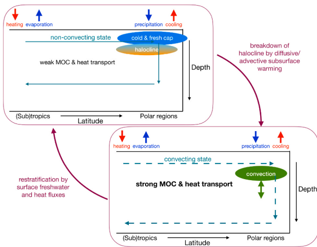
Fig. 9. Sketch to describe the mechanism of the Convection-Restratification variability. Starting in a non- or weakly convecting state, advective (wind-driven) or diffusive warming of the subsurface ocean causes convection and breaks down the halocline. The convective state increases the strength of the AMOC. Through advective and/or diffusive heat and salt fluxes, restratification occurs, which in turn reduces the density at the surface waters eventually causing the transition back to the non-convecting state (details in Winton and Sarachik (1993)).
