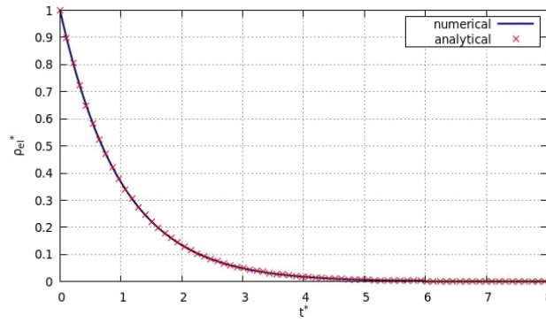
Fig. 2: Charge relaxation in benzene. Analytical and numerical solutions for the evolution of the charge density at the center of the cross section.
