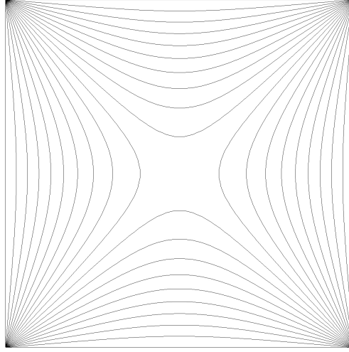
Fig. 6: Laminar flow electrification - non-uniform charge at the boundary. Contour plots of the charge density distribution at steady state and at the cross section ( yz plane) with x = 0 . The plot depicts 20 iso-contours uniformly distributed between \rho_{el}^* = 0.11 (close to the left and right walls) and \rho_{el}^* = 0.98 (close to the top and bottom walls).
