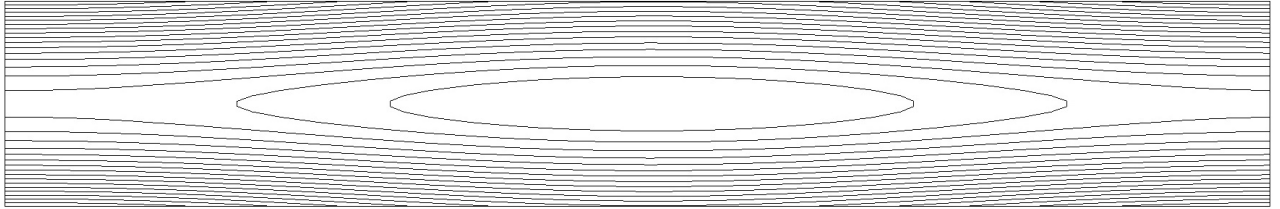
Fig. 7: Laminar flow electrification - non-uniform charge at the boundary. Contour plots of the charge density distribution on the x - y plane at steady-state. The plot depicts 20 iso-contours uniformly distributed between \rho_{el}^* = 0.41 and \rho_{el}^* = 1 .
