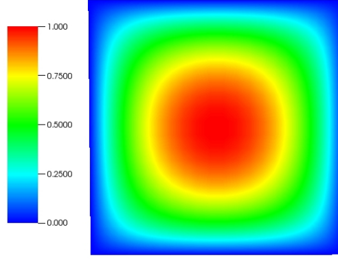
Fig. 1: Charge relaxation in benzene. Colormap of the initial charge density \rho_{el,0}^* at the cross section of the duct. The peak of the charge density, (\rho_{el,0})_{\max} , is located at the center of the cross section.
