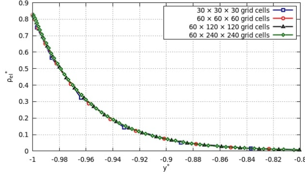
Fig. 5: Laminar flow electrification - uniform charge at the boundary. Profiles of the charge density along the y direction at t^* = 5.0 and z = 0 computed with four different grids.
