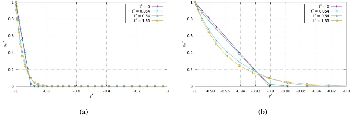
Fig. 3: Laminar flow electrification - uniform charge at the boundary. Charge density profile along the y direction at four different times and z = 0 . The right plot is a zoom near the wall.
