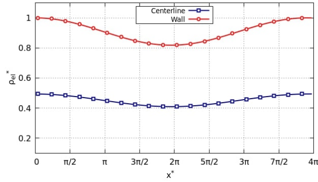
Fig. 8: Laminar flow electrification - non-uniform charge at the boundary. Charge density distribution at steady state along the centerline and at the top and bottom walls.
