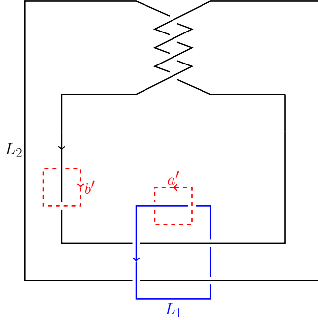
FIGURE 5. The 2-component m -Whitehead link W_m = L_1 \cup L_2 (for m = 2 )
