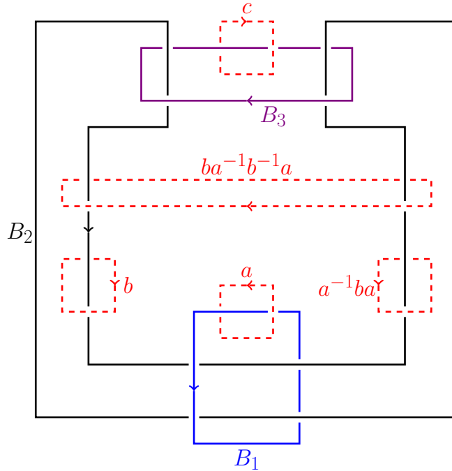
FIGURE 4. The Borromean rings B = B_1 \cup B_2 \cup B_3
