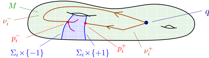
FIGURE 3. The cell decomposition of M
