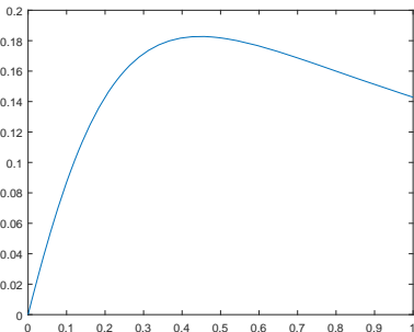
Figure 5. Graph of a Haldane function
