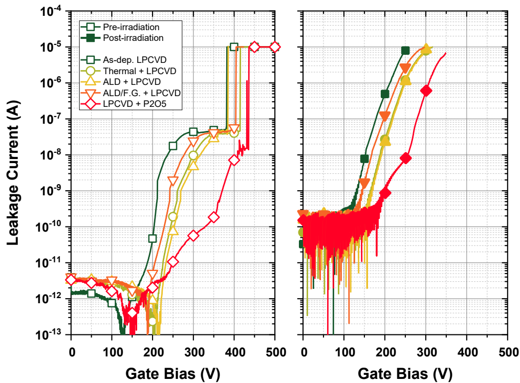
Fig. 2. Comparison of TID MOSCAP I-V response before (left) and after (right) irradiation. Measurements were carried out at 23^\circ\text{C} and device area of 2.1 \times 10^{-5} \text{ cm}^2
