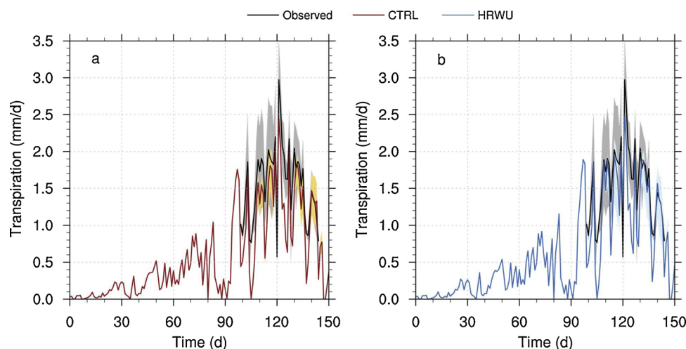
Fig. 10. (a) Time evolution of the measured and simulated transpiration fluxes for the CTRL model at Selhausen minirhizotron facility based on SOIL-SCEN1, and with the envelope defined according to three root distributions depicted in Fig. 2b. (b) Same as (a) for the HRWU model.
