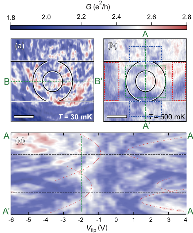
FIG. 3. (Color online) SGM images of the QR at low charge-carrier density, close to the neutrality point. (a),(b) SGM map at V_g = +18 V, B = 0.7 T, V_{\text{tip}} = -2 V, and T = 30 and 500 mK, respectively. Continuous lines indicate the position of the QR. The scale bars correspond to 400 nm. (c) Plot of the conductance vs V_{\text{tip}} and the tip position along the AA' green dashed line in Fig. 3(b). The positions of both QR apertures are given by the black dashed lines. Red dashed lines correspond to a Gaussian fit to the data, and highlight Coulomb resonances.
