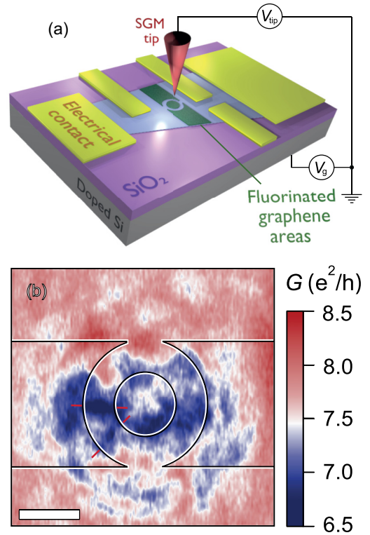
FIG. 2. (Color online) SGM imaging of the QR. (a) SGM experimental setup: the graphene QR is defined by fluorination (green regions) and lies on an oxidized doped Si substrate, used as a back gate. The yellow areas correspond to ohmic contacts on top of the graphene flake. A metallic tip is approached close to the QR, with an applied bias V_{tip} , and is scanned to produce a SGM map of the device conductance. (b) SGM conductance map obtained at large charge-carrier concentration ( n = 7.2 \times 10^{12} \text{ cm}^{-2} ; V_g = -5 V), V_{tip} = -2 V, B = 30 mT, and T = 30 mK. The continuous lines delineate the position of the QR. The red dashes highlight two examples of conductance fringes inside the QR arms. The scale bar represents 400 nm.
