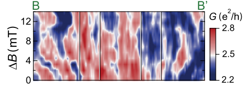
FIG. 4. (Color online) SGM line profile, measured along the BB' green dashed line in Fig. 3(a), as a function of the magnetic field ( V_{\text{tip}} = -2 V, V_g = +18 V and B = 0.7 T). Vertical lines correspond to the inner and outer limits of the QR.
