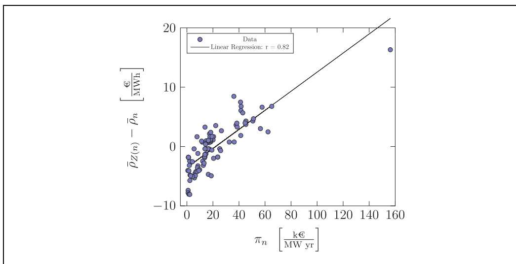
Figure 4. Difference between the average zonal and nodal prices as a function of the optimal capacity price.
